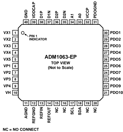
Figure 3. Pin Configuration
