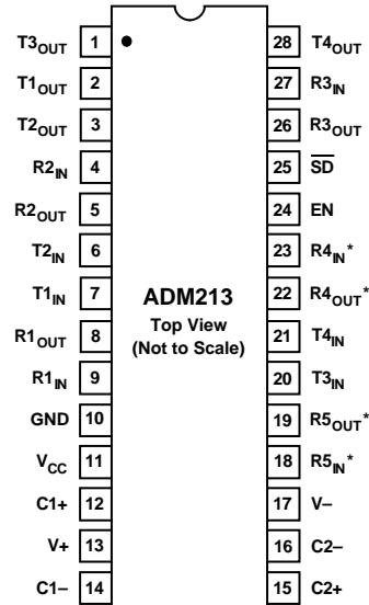
Figure 13. ADM213 SOIC/SSOP Pin Configuration
