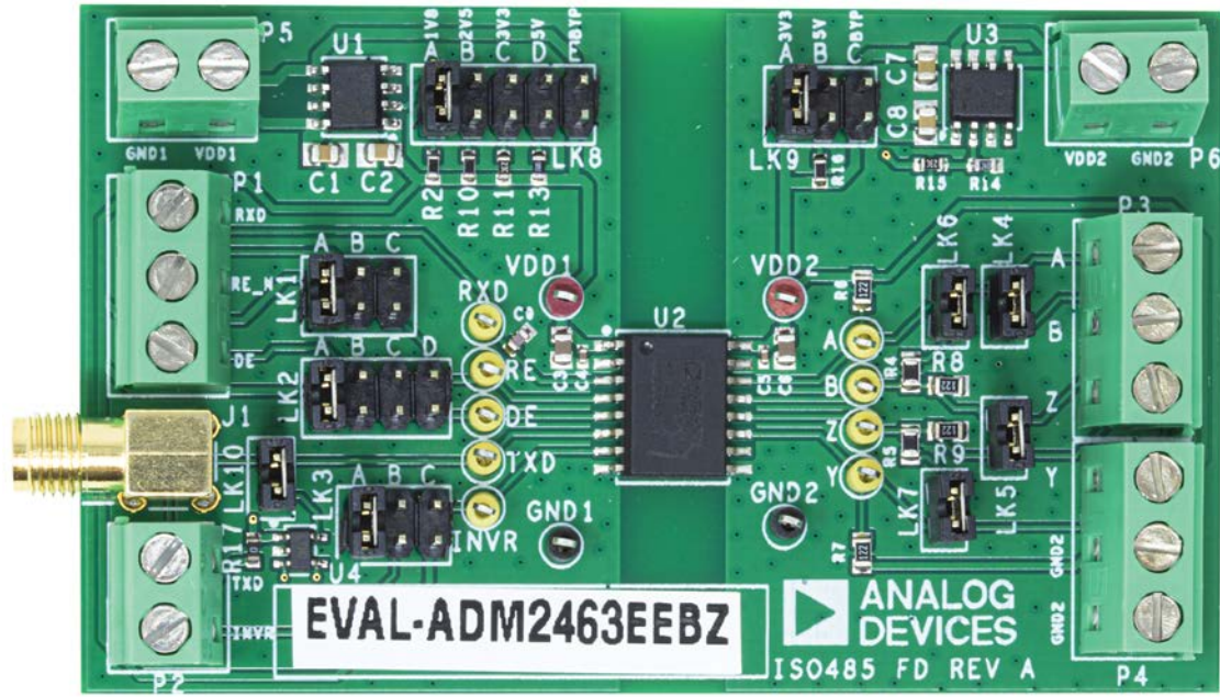
Figure 1. EVAL-ADM2463EEBZ
