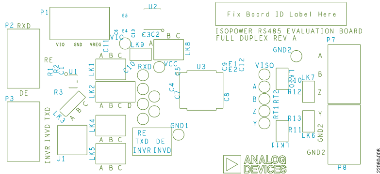
Figure 9. EVAL-ADM2867EEBZ, Silkscreen
