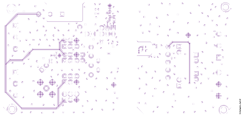
Figure 8. EVAL-ADM2867EEBZ, Layer 2
