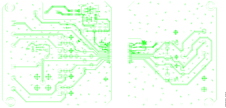
Figure 7. EVAL-ADM2867EEBZ Component Side, Layer 1
