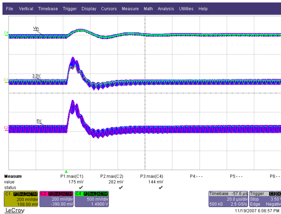
Figure 18. Transient 100% to 50% load: Ch1 = 3.3 V, Ch2 = 5.0 V, Ch4 = Vin @ 16.0 V
