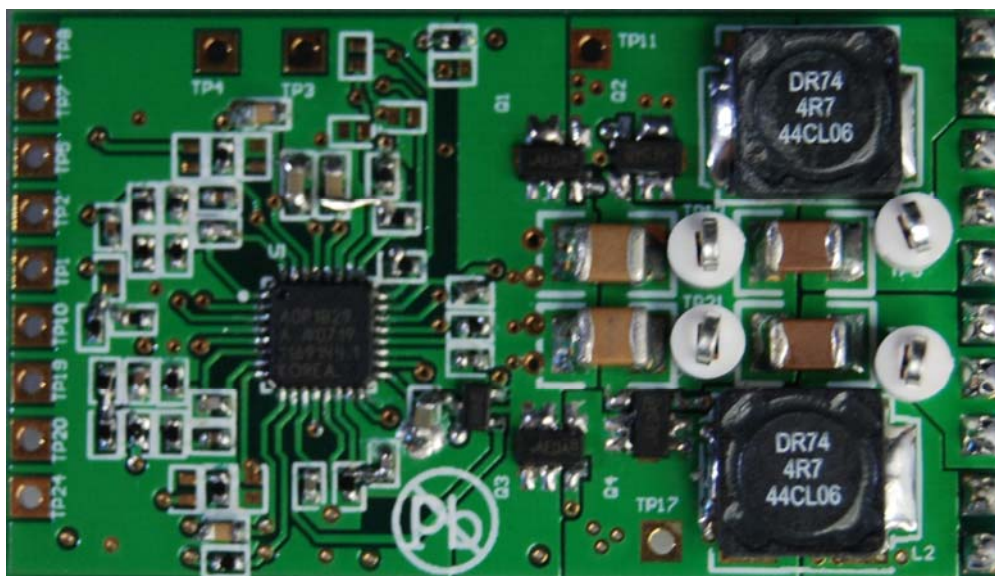
Figure 1. ADP1829 Evaluation Board
