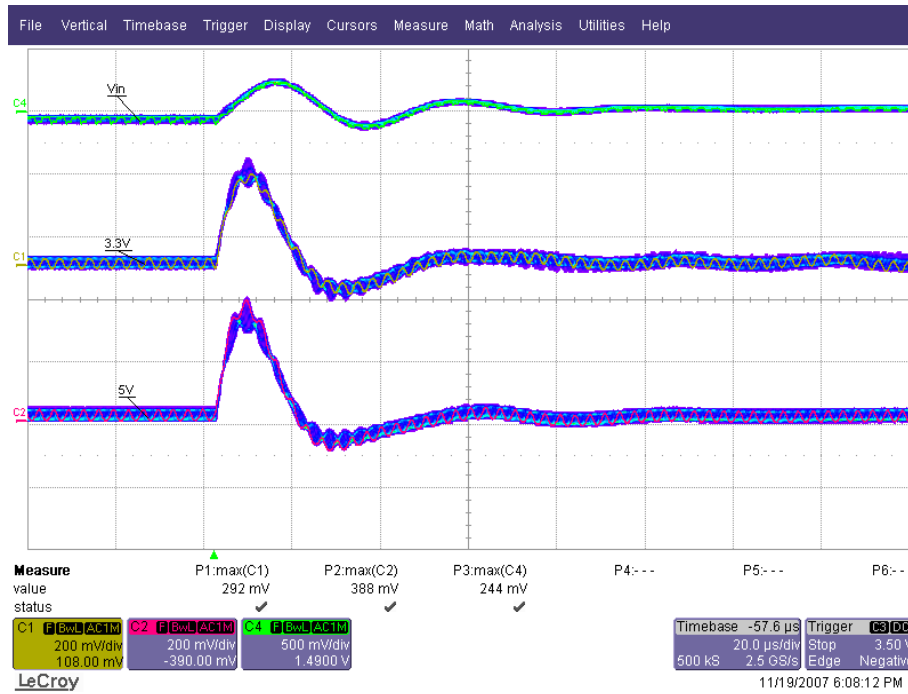
Figure 17. Transient 100% to 50% load: Ch1 = 3.3 V, Ch2 = 5.0 V, Ch4 = Vin @ 8.0 V
