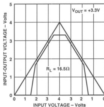
Figure 9. Power-Up/Power-Down
