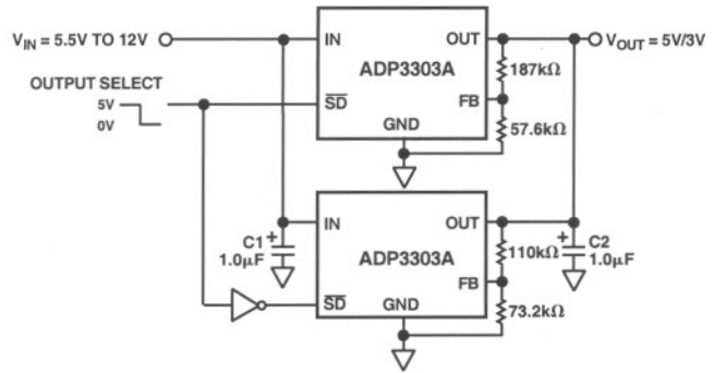
Figure 23. Crossover Switch
