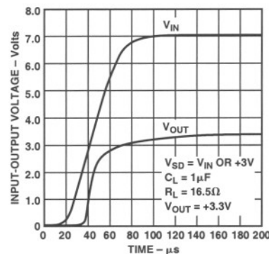
Figure 10. Power-Up Transient
