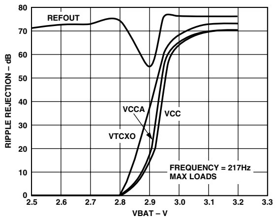
FREQUENCY = 217Hz MAX LOADS TPC 12. Ripple Rejection vs. Battery Voltage
