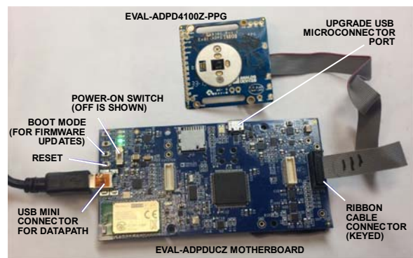
Figure 5. Connect the EVAL-ADPDCUZ to the EVAL-ADPD4100Z-PPG
