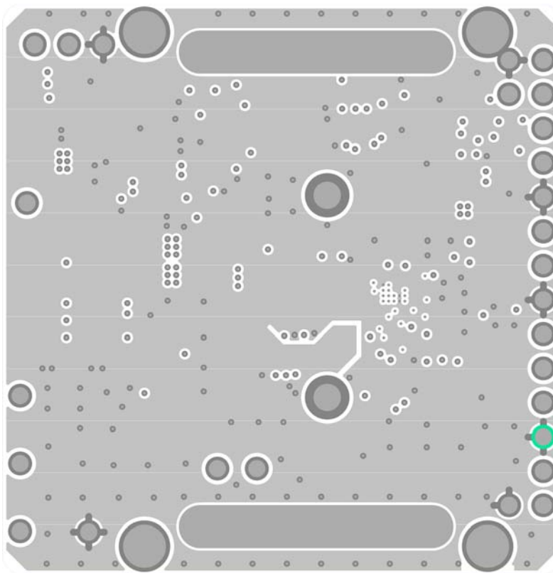
Figure 14. Layer 2, Ground
