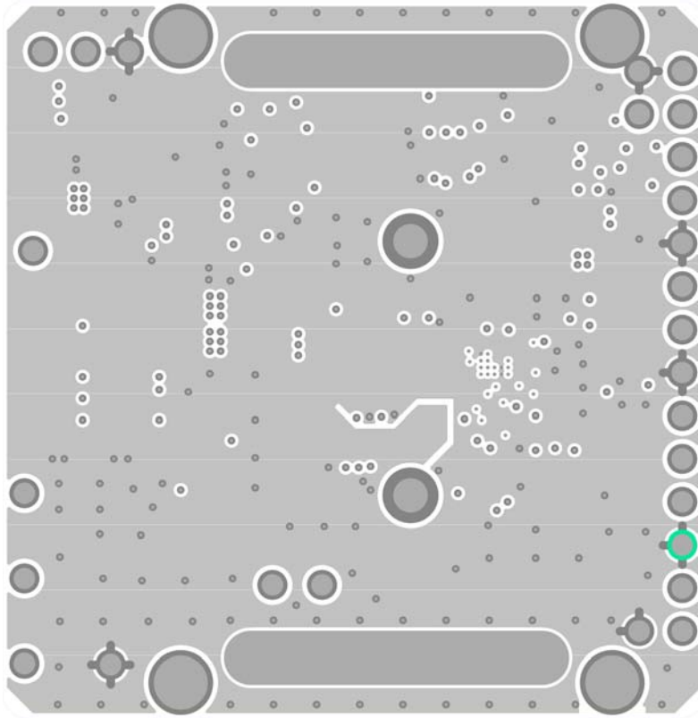
Figure 17. Layer 5, Ground
