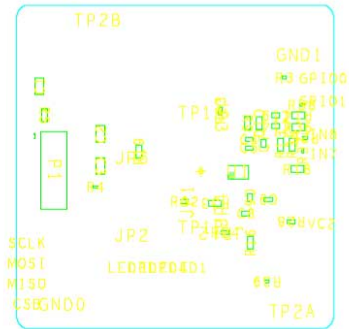
Figure 18. EVAL-ADPD4200Z-PPG Top and Bottom Silkscreen View
