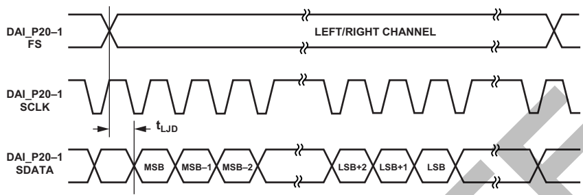
Figure 33. Left-Justified Mode
