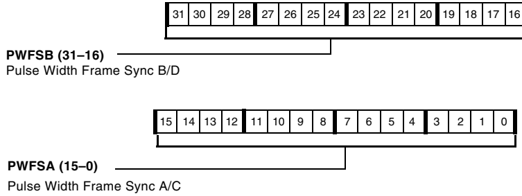
Figure A-63. PCG_PW x Registers (Normal Mode)
