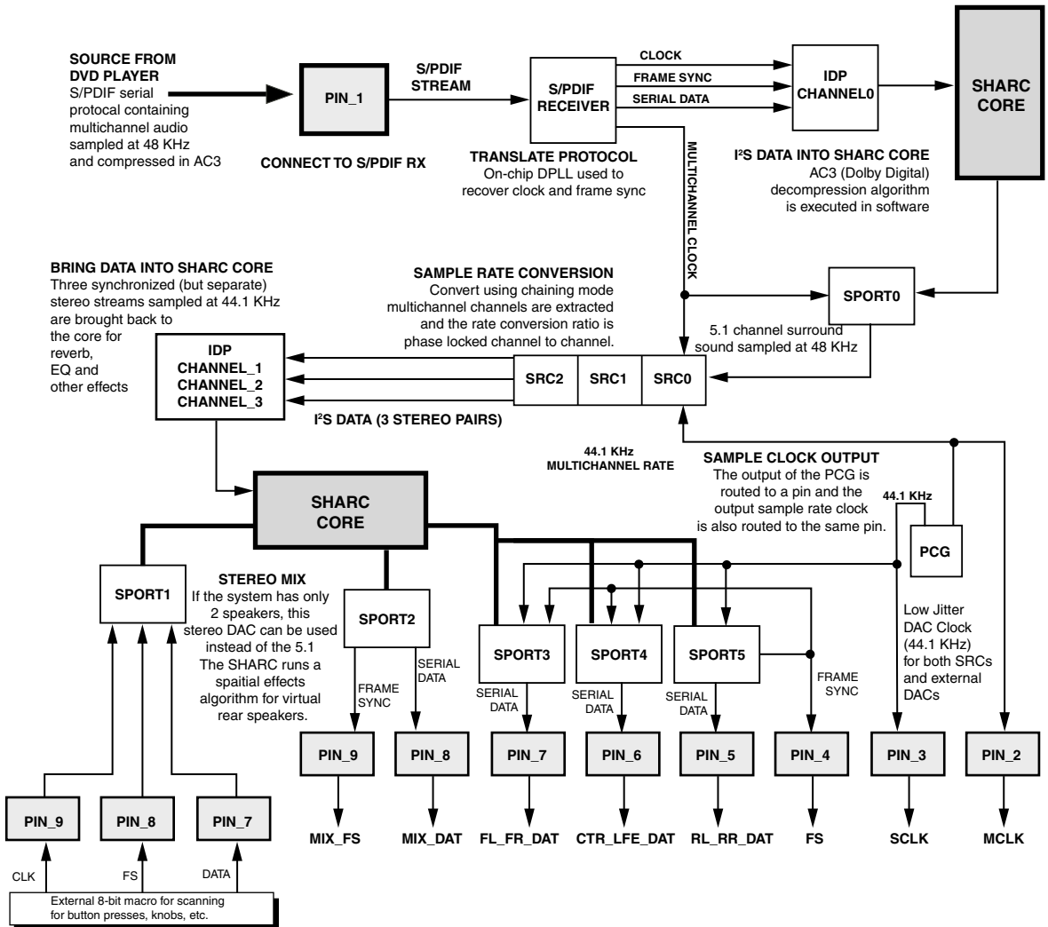
Figure 6-16. DAI Example
