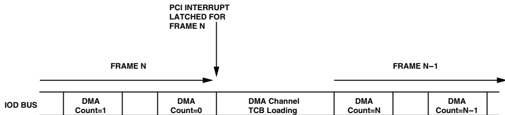
Figure 2-4. DMA Chaining
