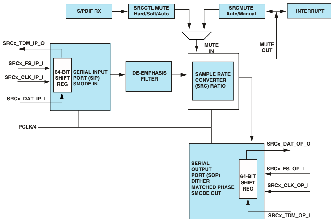
Figure 9-1. Sample Rate Converter Block Diagram
