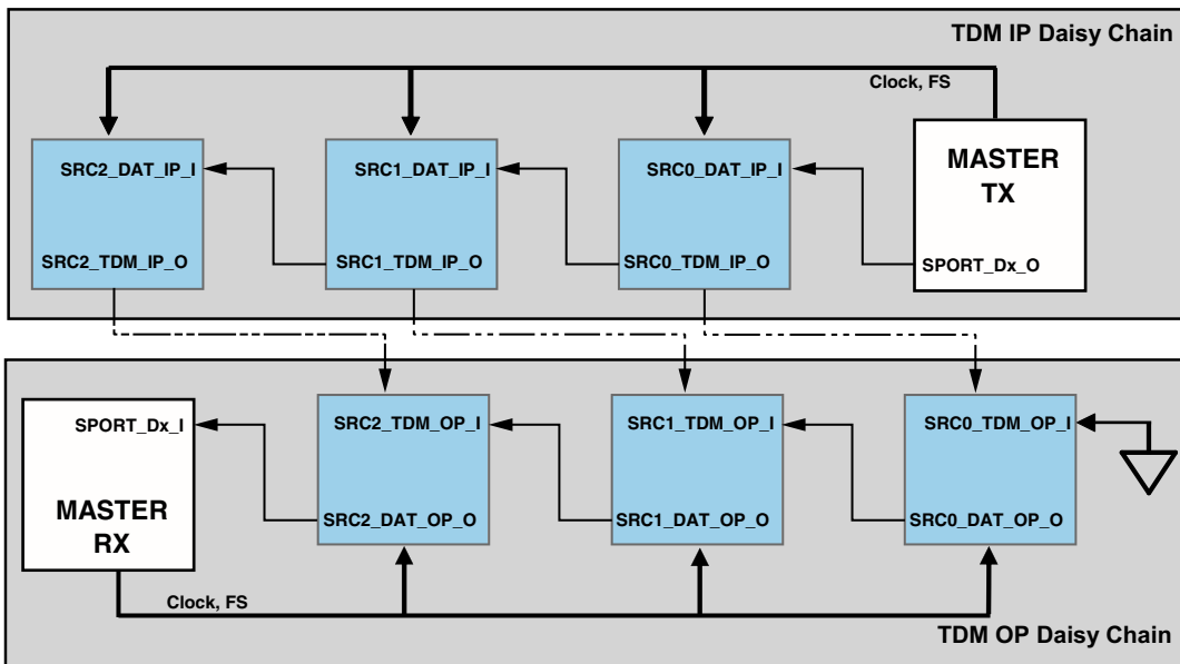
Figure 9-4. TDM Input/Output Modes
