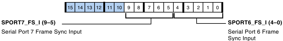
Figure A-32. SRU_FS4 Register (RW)
