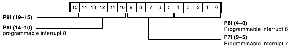
Figure B-2. PICR1 Register
