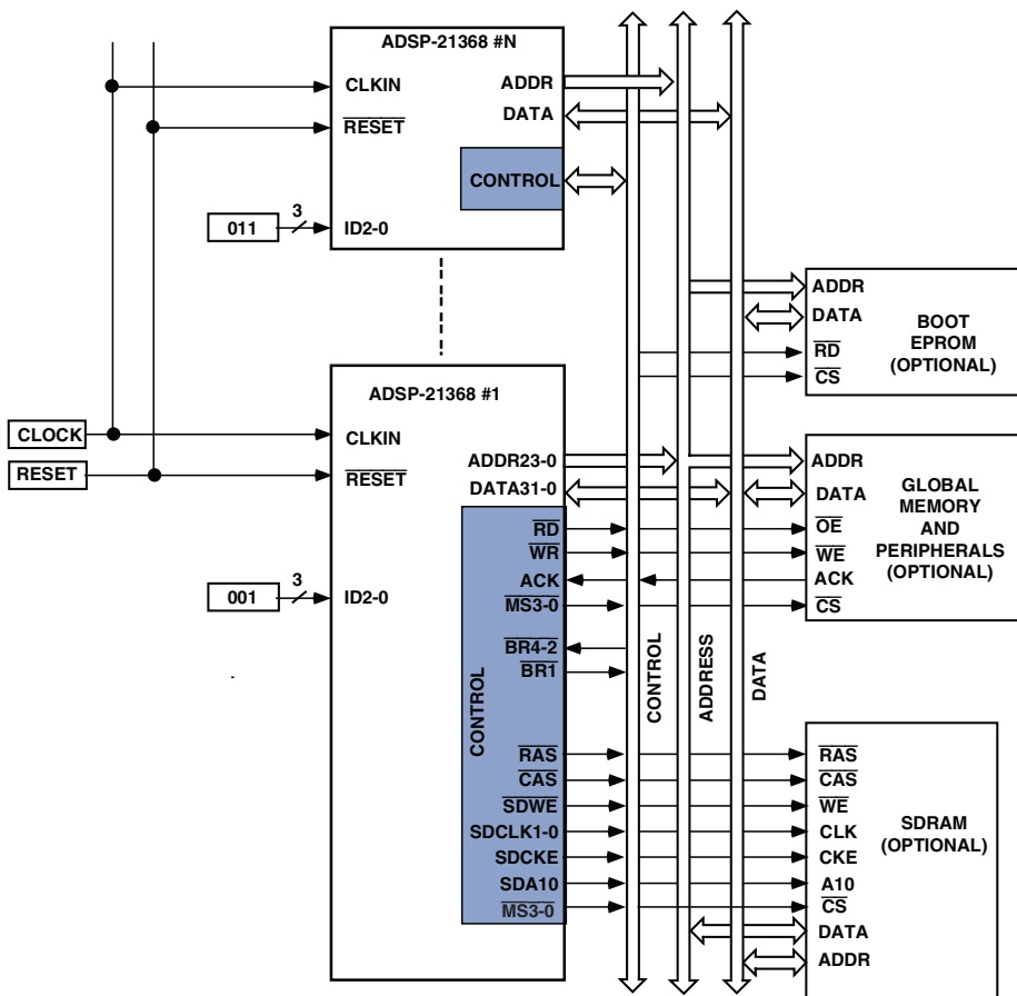
Figure 3-12. ADSP-21368 Shared Memory System
