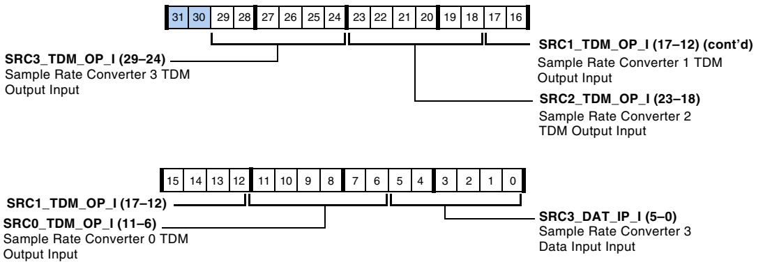
Figure A-24. SRU_DAT3 Register (RW)
