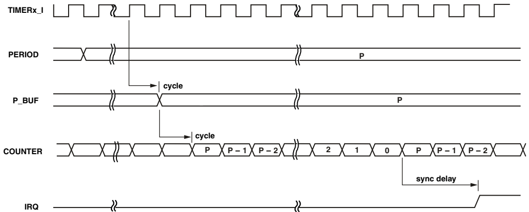
Figure 13-8. EXT_CLK Timing
