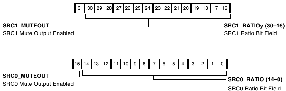
Figure A-59. SRCRAT0 Register
