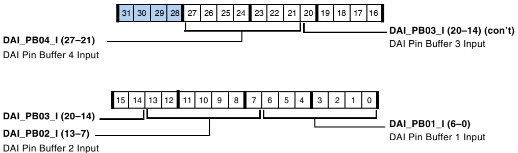
Figure A-33. SRU_PIN0 Register (RW)
