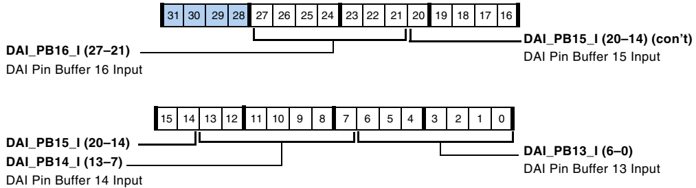
Figure A-36. SRU_PIN3 Register (RW)
