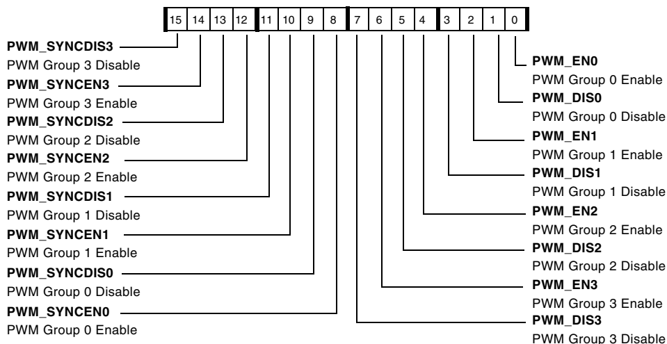
Figure A-13. PWMGCTL Register
