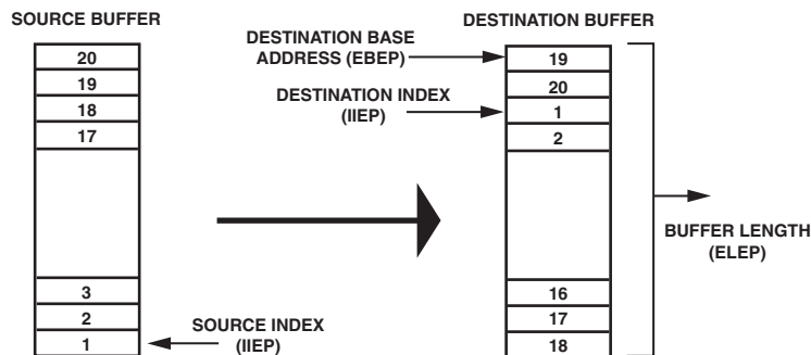
Figure 3-18. Circular Buffering Write DMA
