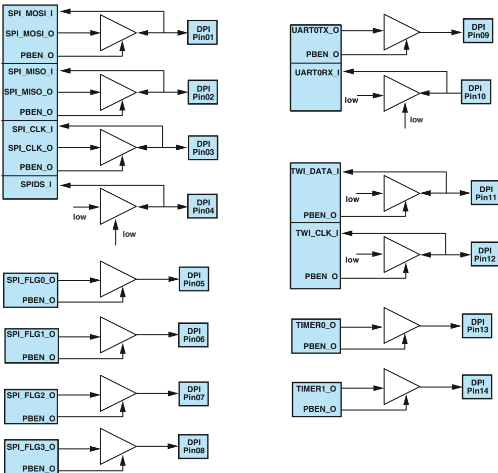
Figure 6-15. DPI Default Routing
