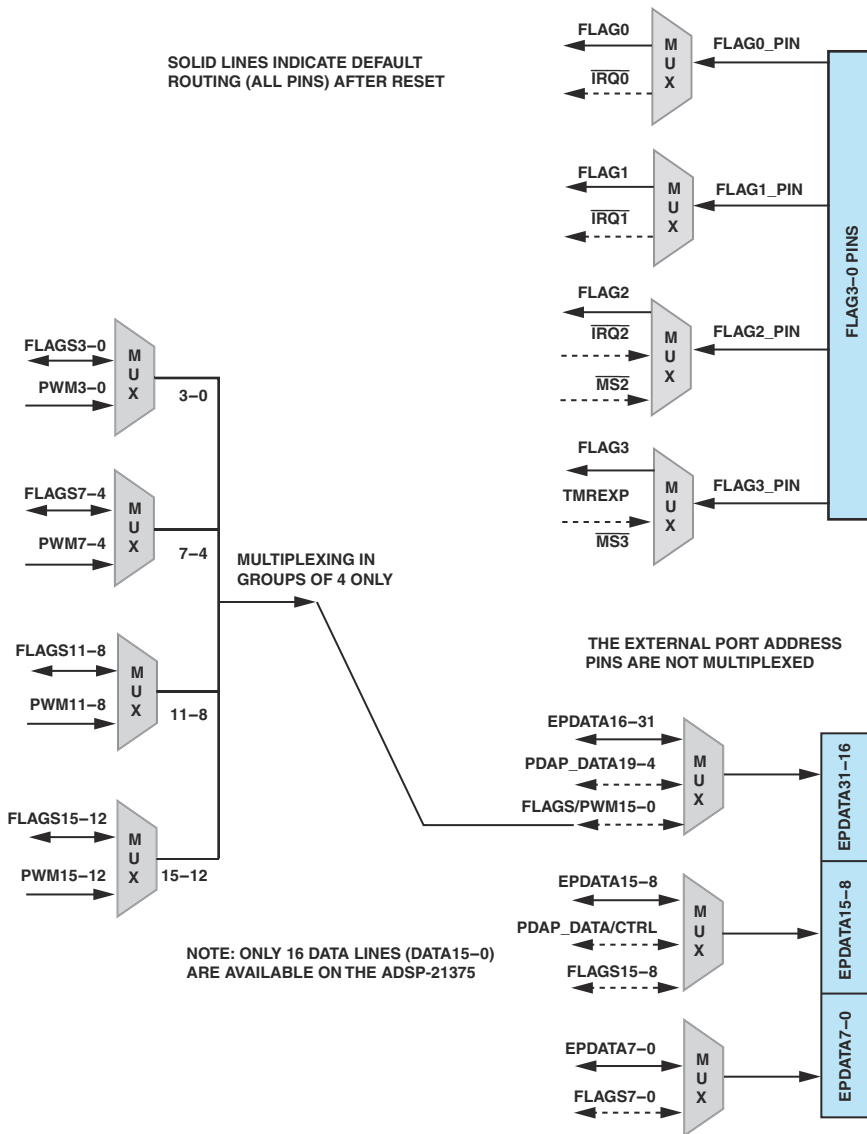
Figure 17-9. Pin Multiplexing
