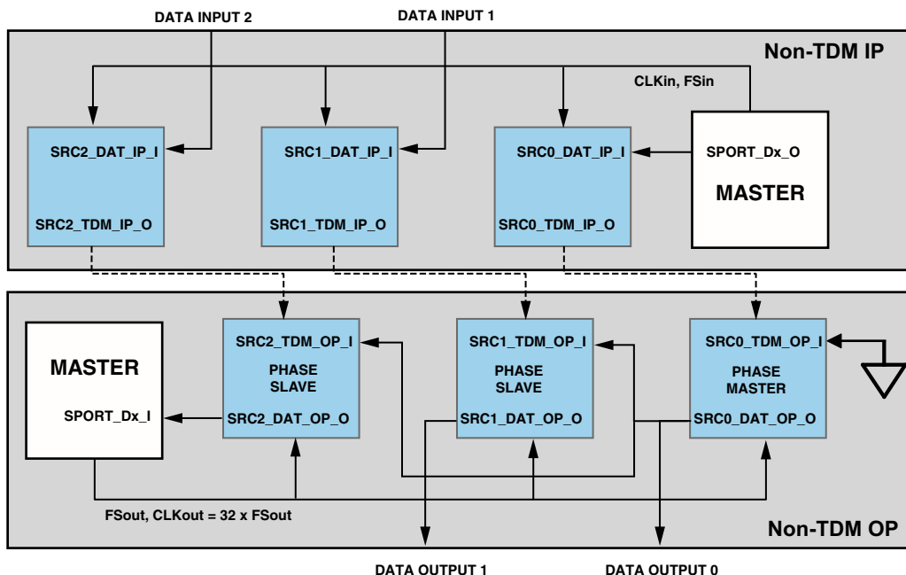
Figure 9-5. Typical Configuration for Matched-Phase Mode Operation
