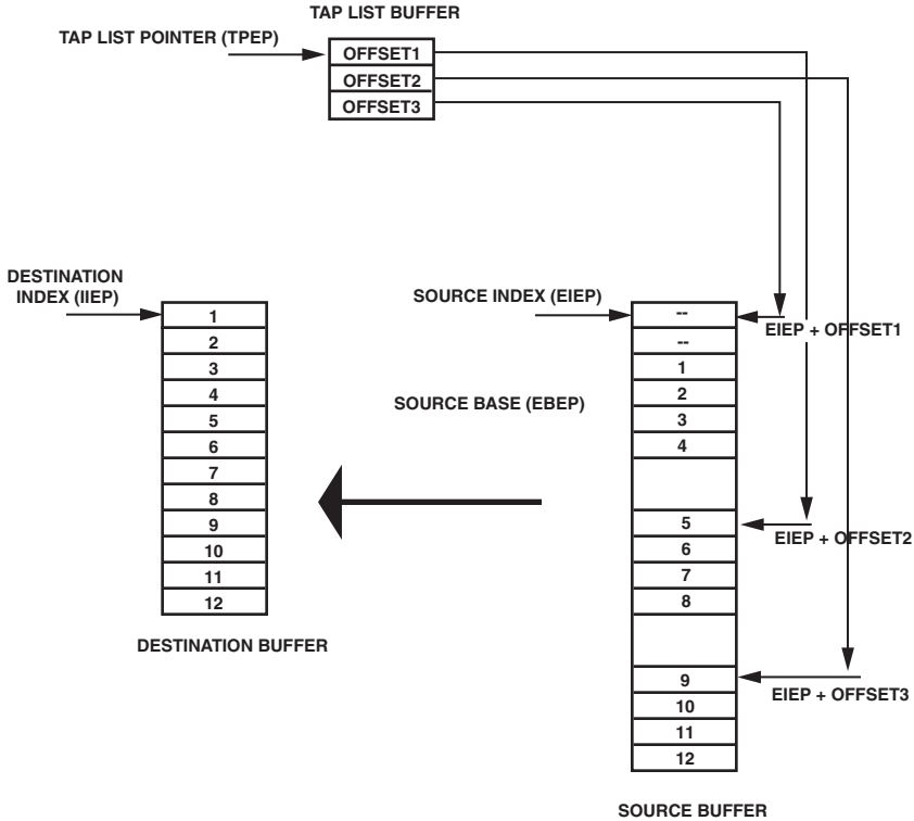
Figure 3-21. Gather DMA (Reads)
