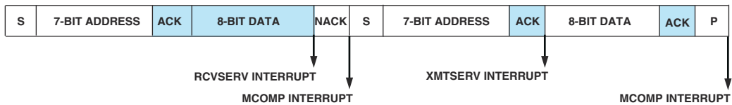
Figure 15-12. Receive/Transmit Data Repeated Start
