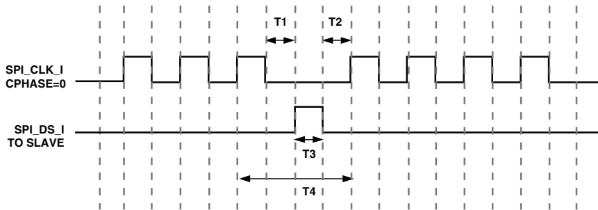
Figure 12-7. SPICLK Timing
