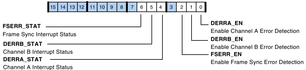
Figure A-52. SPERRCTLx Register
