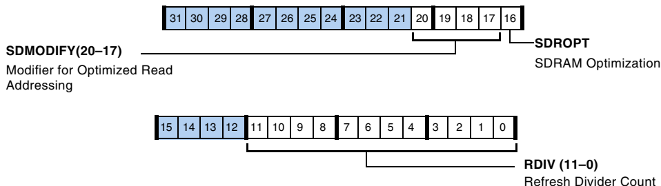
Figure A-10. SDRRC Register
