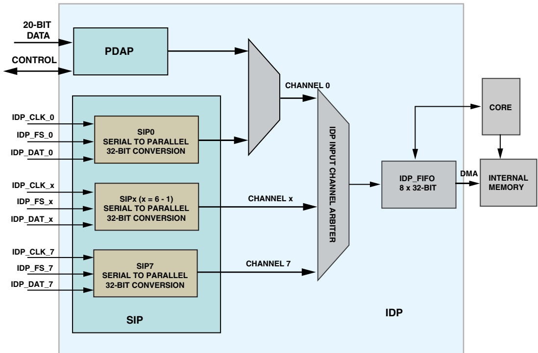
Figure 8-1. Input Data Port
