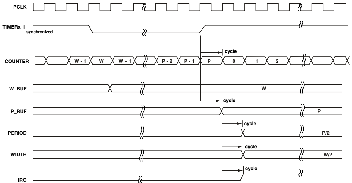
Figure 13-6. WDTI_CAP Timing (Period Count = 1)
