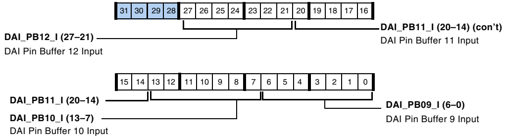
Figure A-35. SRU_PIN2 Register (RW)
