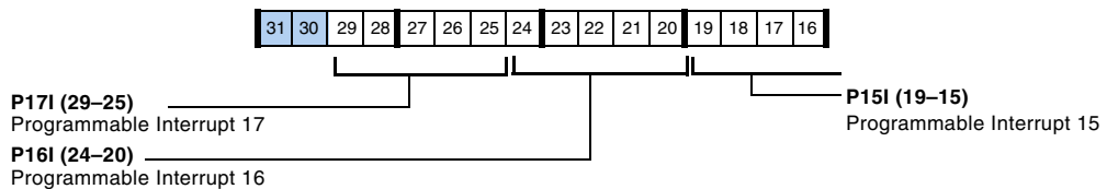
Figure B-2. PICR1 Register
