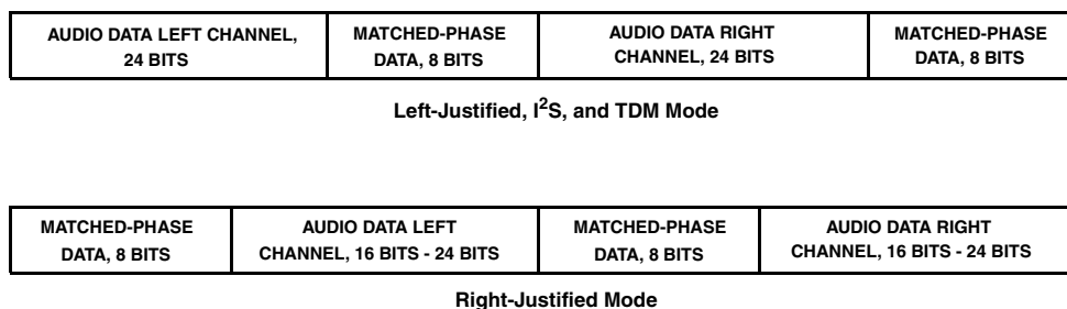
Figure 9-6. Matched-Phase Data Transmission
