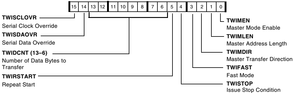
Figure A-101. TWIMCTL Register
