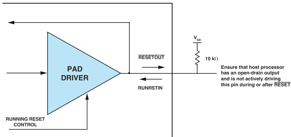
Figure 17-1. RESETOUT Pin Multiplexed with RUNRSTIN
