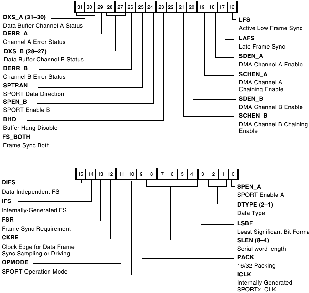
Figure A-48. SPCTLx Register for Serial Mode
