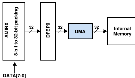
Figure 17-3. External Port Data Packing
