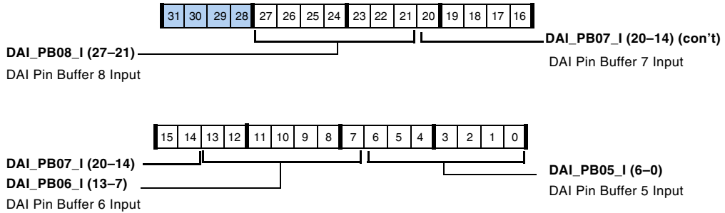
Figure A-34. SRU_PIN1 Register (RW)
