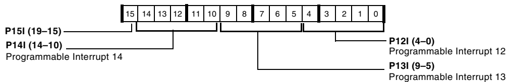
Figure B-3. PICR2 Register
