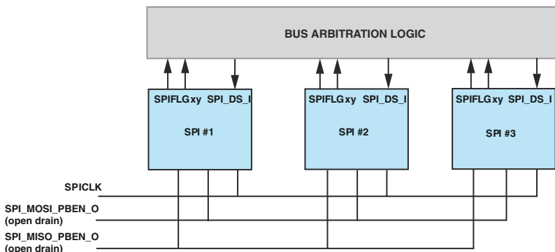
Figure 12-4. Multi Master System
