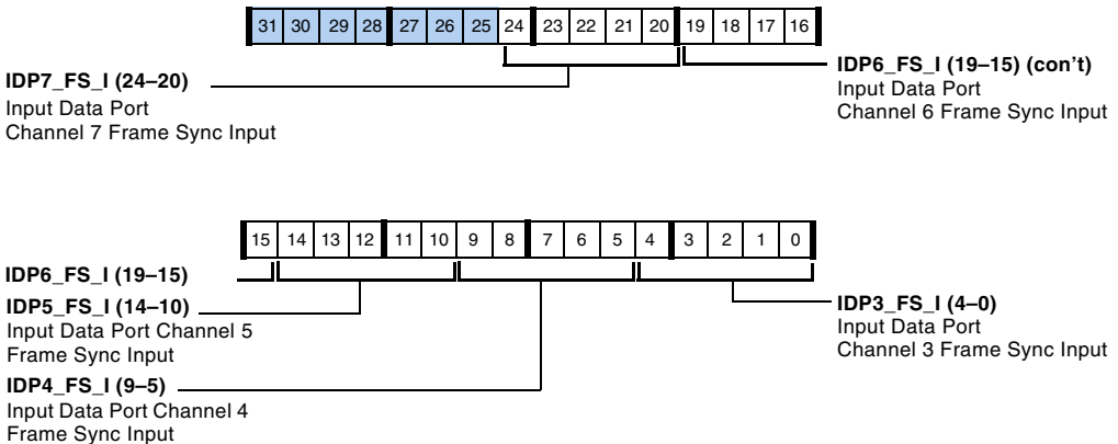
Figure A-31. SRU_FS3 Register (RW)
