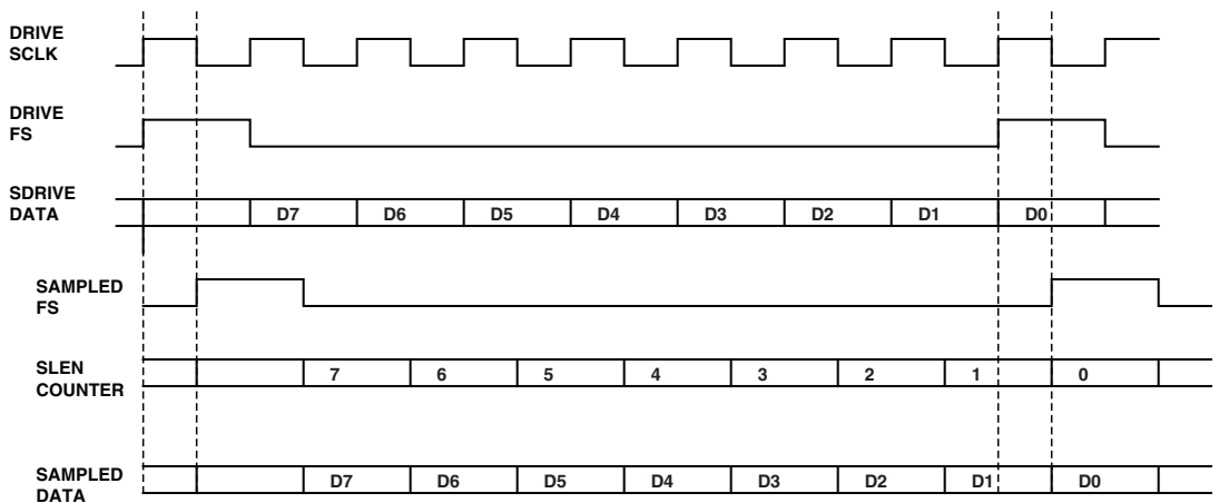
Figure 7-3. Frame Sync and Data Driven on Falling Edge
