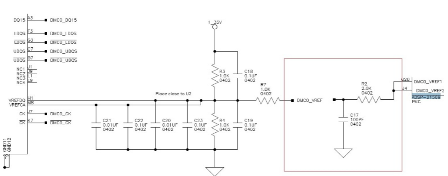
Figure 4. DMC_VREF Filtering Network
