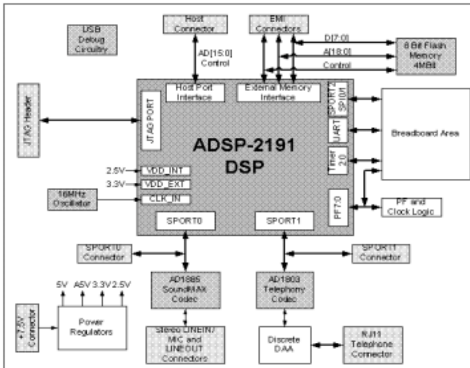
Figure 3-1. System Architecture
