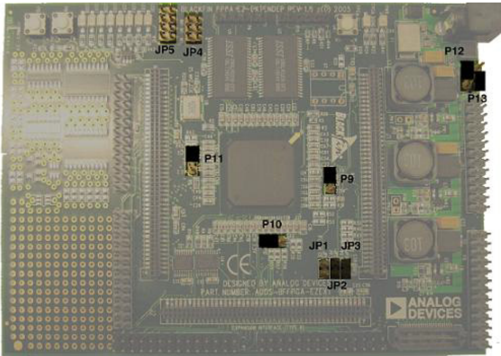
Figure 2-3. Jumper Locations
