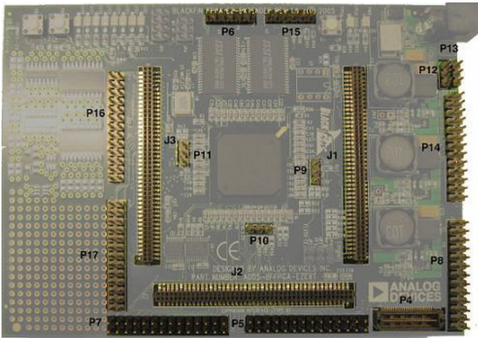
Figure 2-5. Connector Locations
