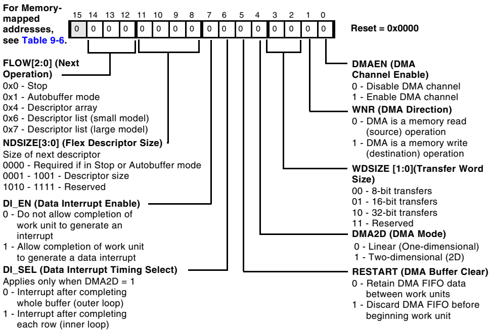
Figure 9-3. Configuration Register
