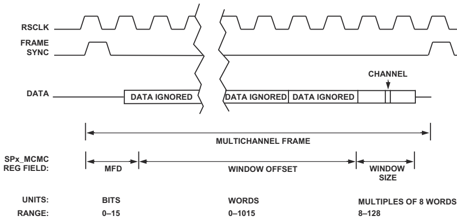
Figure 12-7. Relationships for Multichannel Parameters
