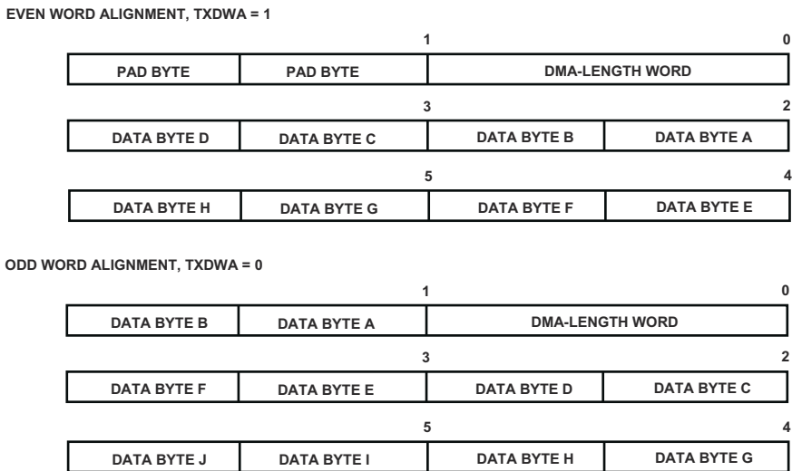
Figure 8-9. TX DMA Data Alignment
