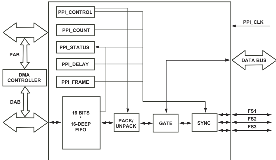
Figure 7-1. PPI Block Diagram
