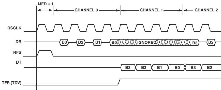
Figure 12-6. Multichannel Operation
