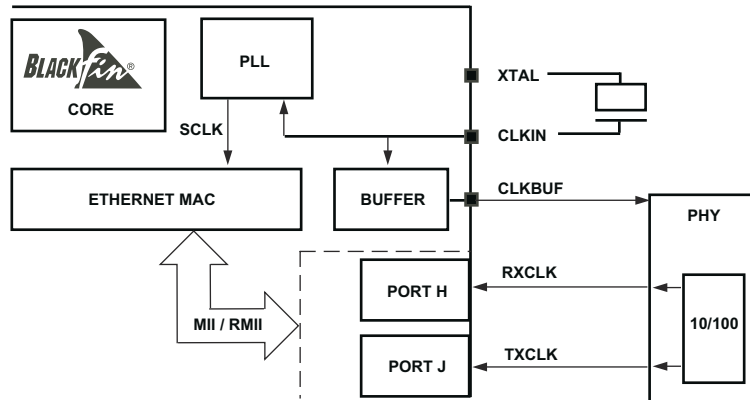
Figure 8-2. Clock Function Diagram
