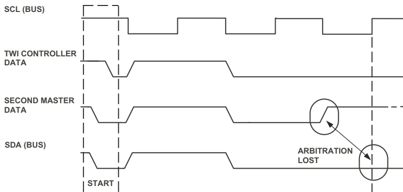
Figure 11-5. TWI Bus Arbitration
