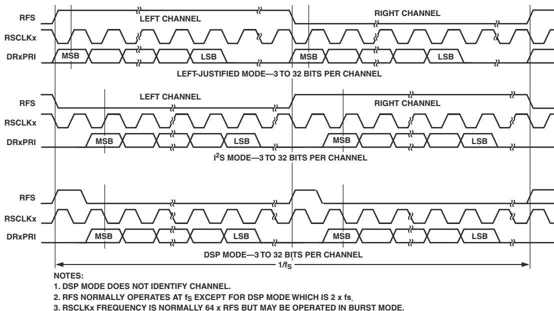
Figure 12-5. SPORT Stereo Serial Modes, Receive
