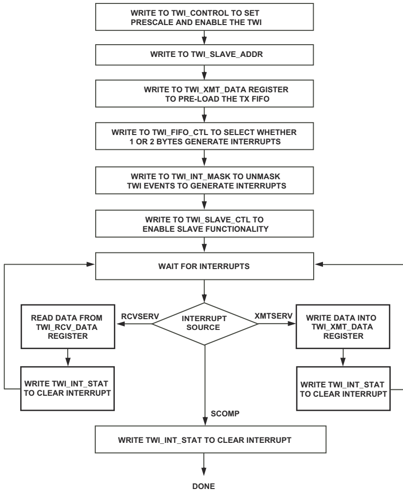
Figure 11-12. TWI Slave Mode
