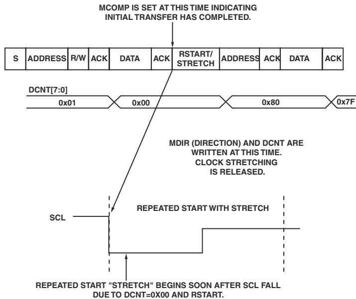
Figure 11-11. Clock Stretching During Repeated Start Condition
