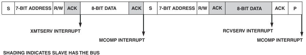
Figure 11-7. Transmit/Receive Data Repeated Start
