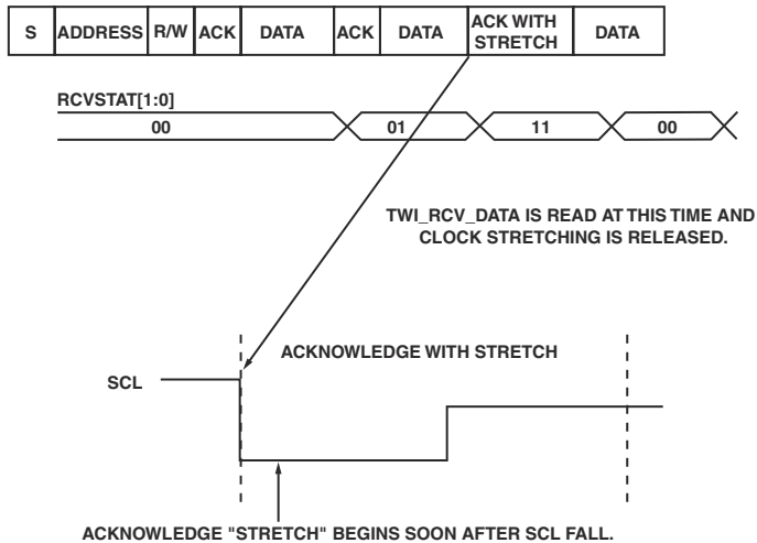
Figure 11-10. Clock Stretching During FIFO Overflow
