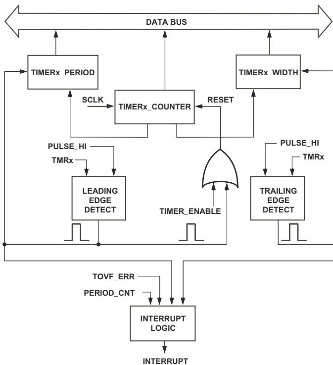
Figure 15-11. Timer Flow Diagram, WIDTH_CAP Mode
