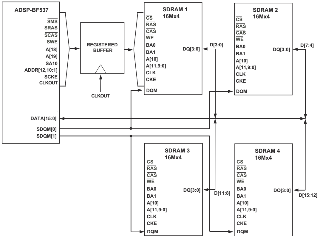
Figure 6-13. SDRAM System Block Diagram, Example 2
