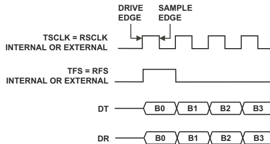
Figure 12-10. Example of TCKFE = RCKFE = 0 , Transmit and Receive Connected
