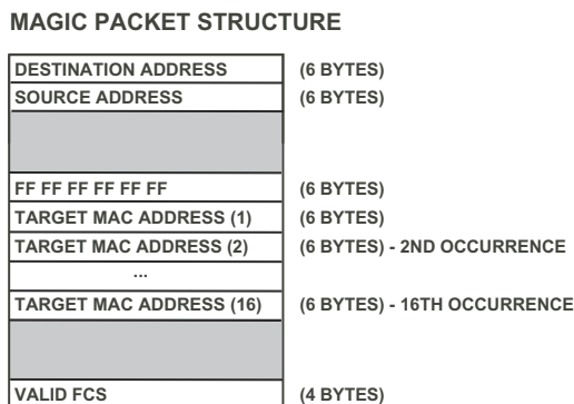
Figure 8-10. Magic Packet Structure
