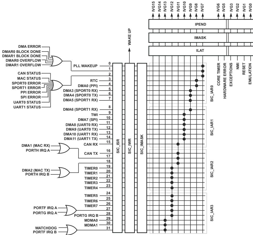
Figure 4-1. Interrupt Routing Overview
