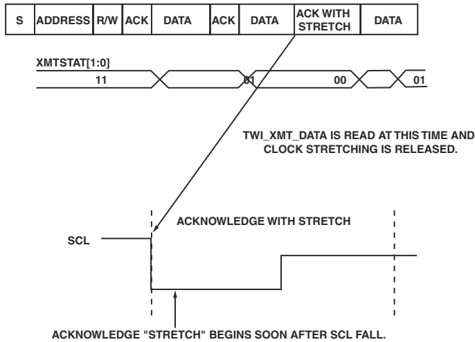
Figure 11-9. Clock Stretching During FIFO Underflow
