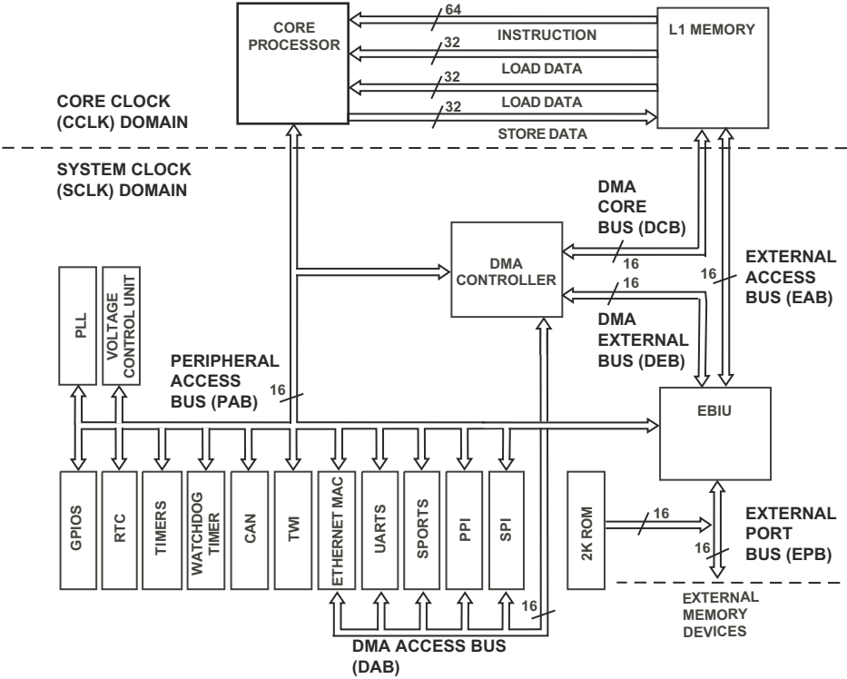
Figure 2-1. Processor Bus Hierarchy
