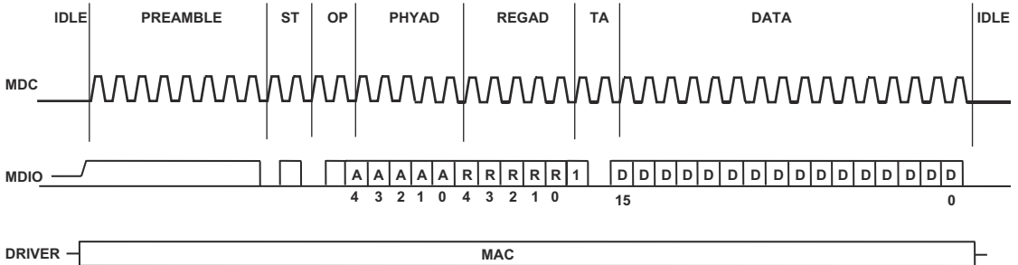
Figure 8-4. Station Management Write
