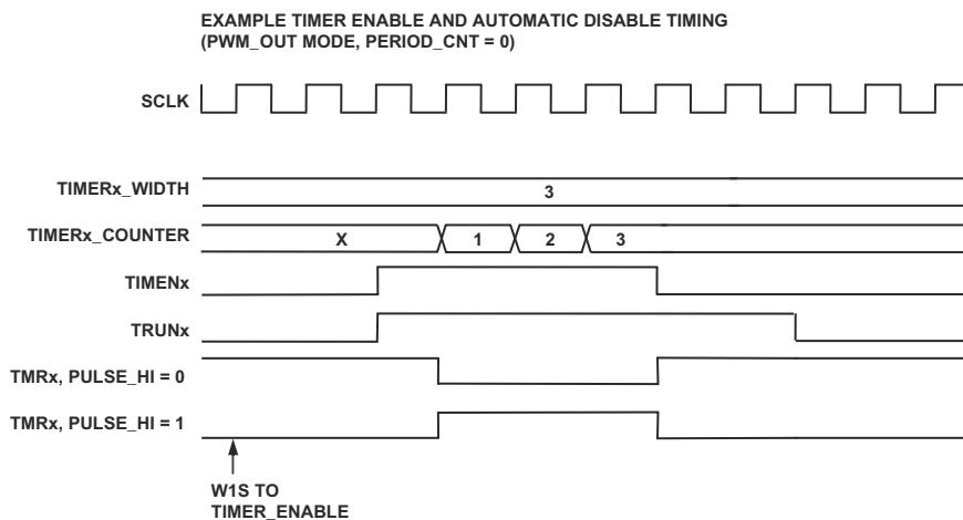
Figure 15-5. Timer Enable and Automatic Disable Timing
