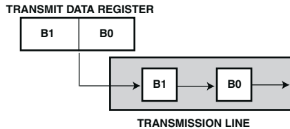
Figure 11-26. Little Endian Byte Order
