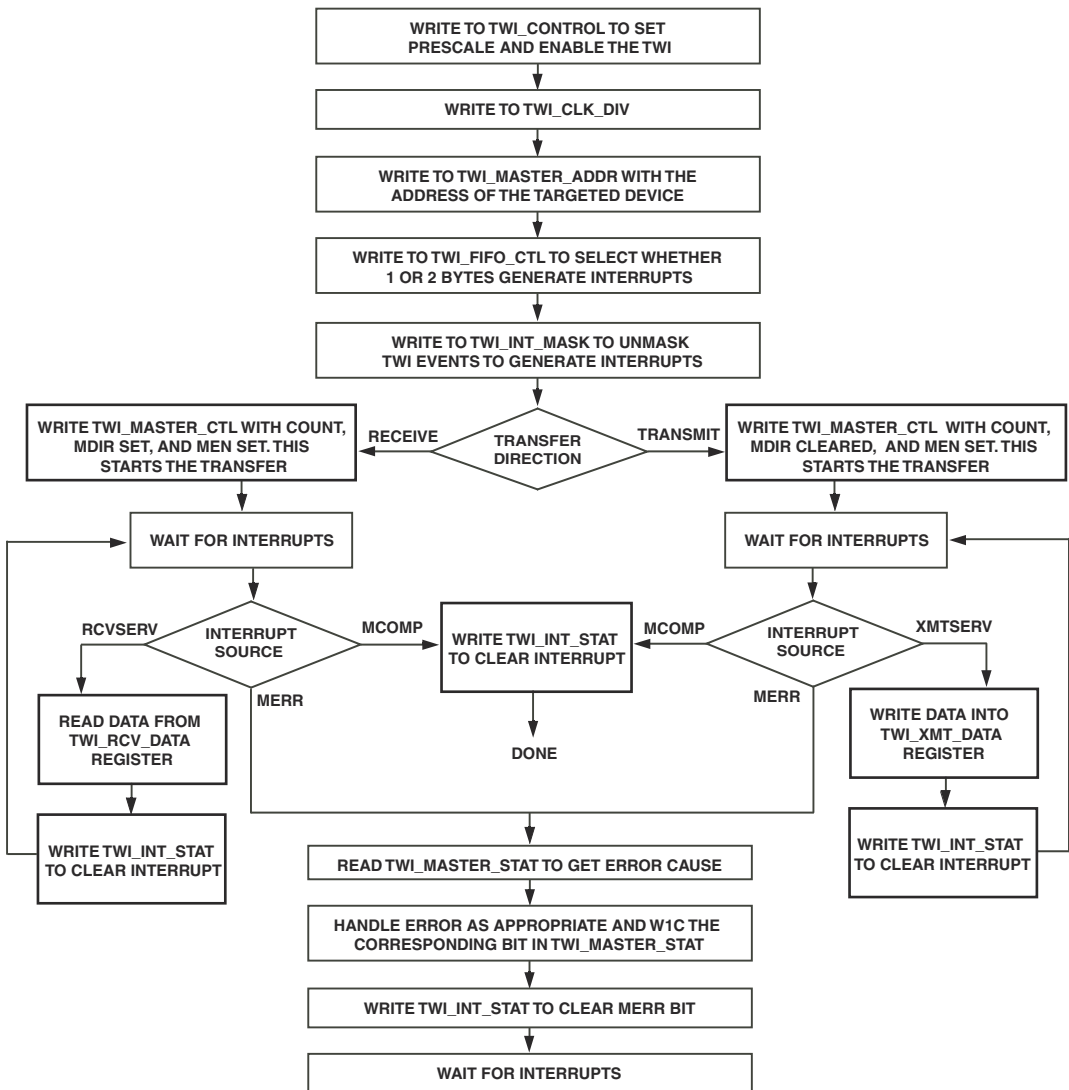
Figure 11-13. TWI Master Mode
