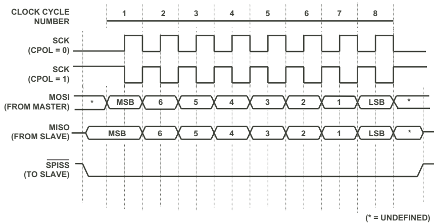
Figure 10-6. SPI Transfer Protocol for CPHA = 0
