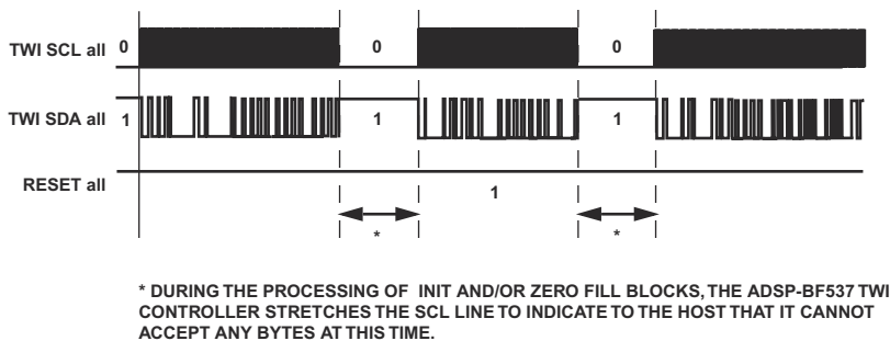
Figure 19-31. TWI Slave Booting
