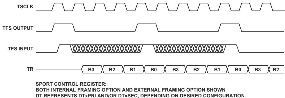
Figure 12-20. SPORT Continuous Transmit, Normal Framing
