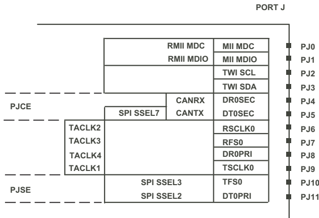
Figure 14-4. Port J Multiplexing Scheme
