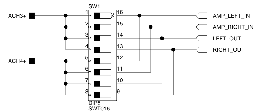
SW1: Oscilloscope Select Switch
