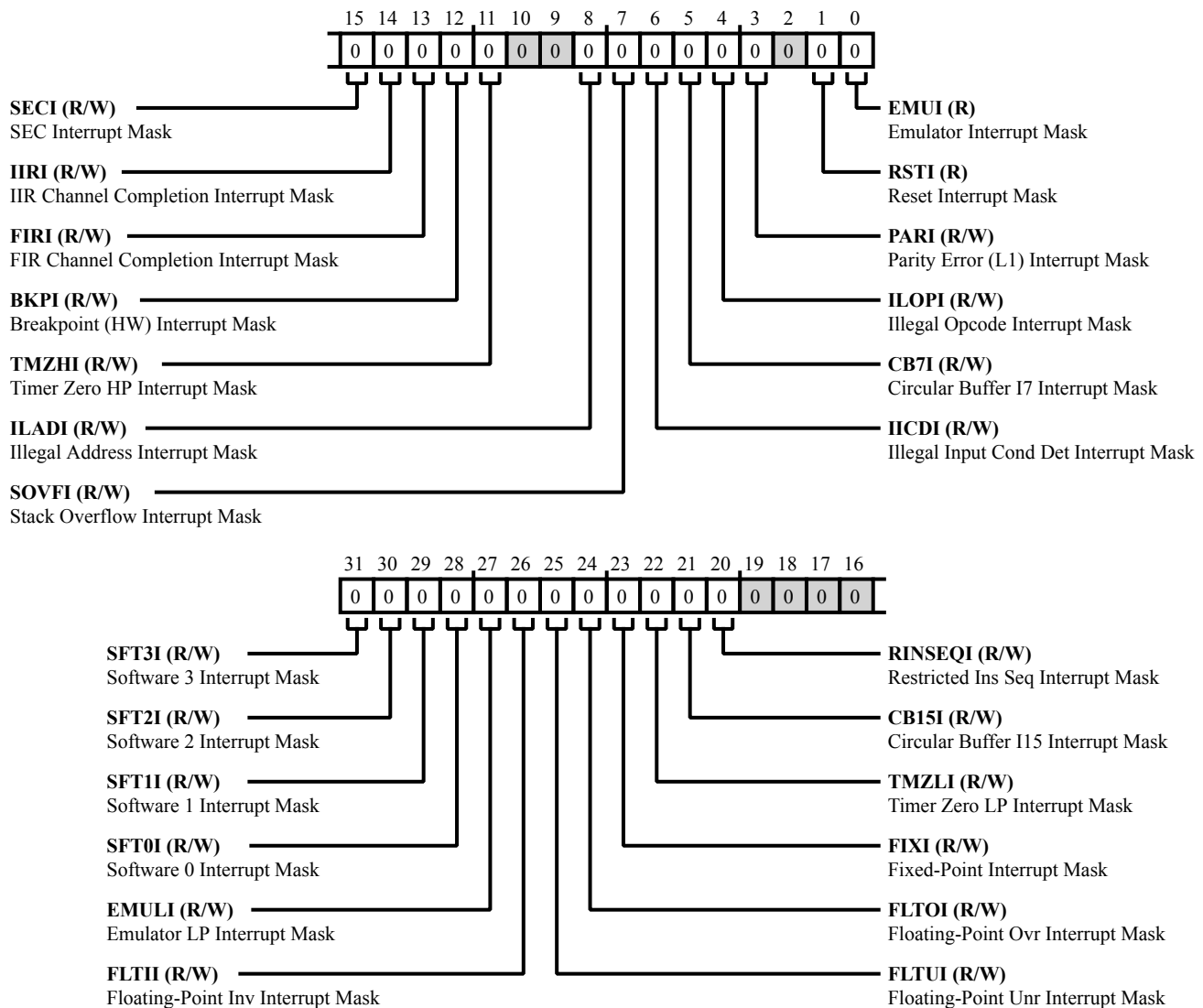
Figure 28-10: REGF_IMASK Register Diagram
