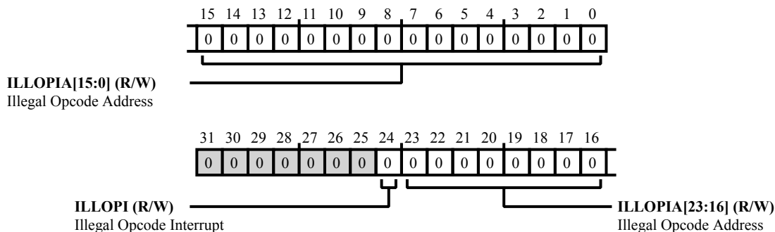
Figure 31-6: SHDBG_DBGREG_ILLOP Register Diagram
