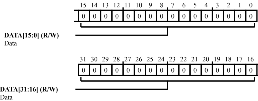
Figure 28-16: REGF_L[n] Register Diagram
