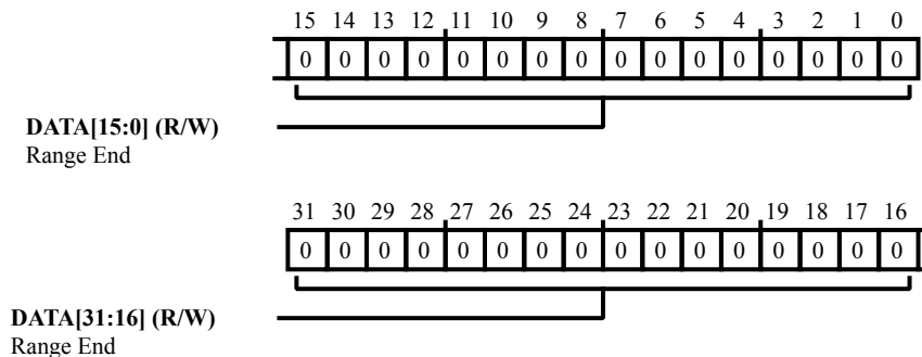
Figure 32-8: SHL1C_RANGE_END3 Register Diagram
