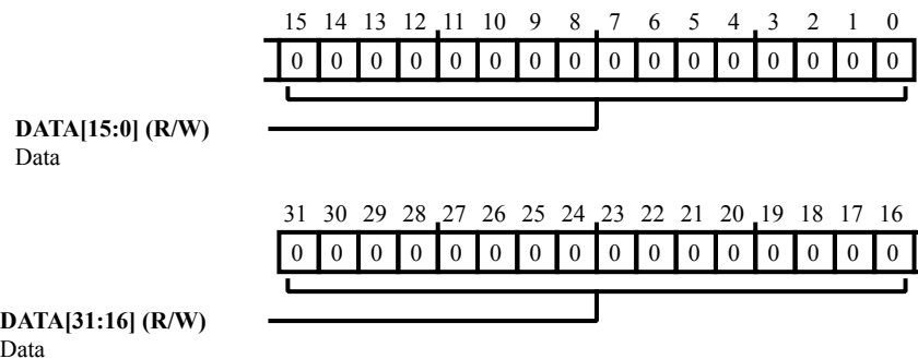
Figure 28-41: REGF_TCOUNT Register Diagram
