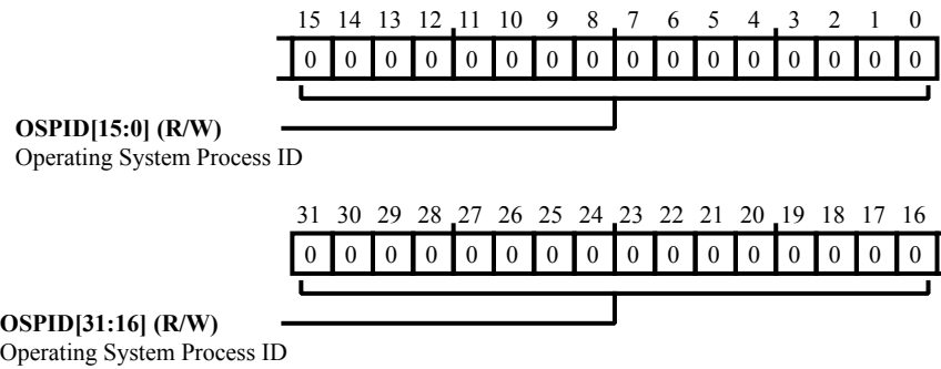
Figure 31-21: SHDBG_OSPID Register Diagram
