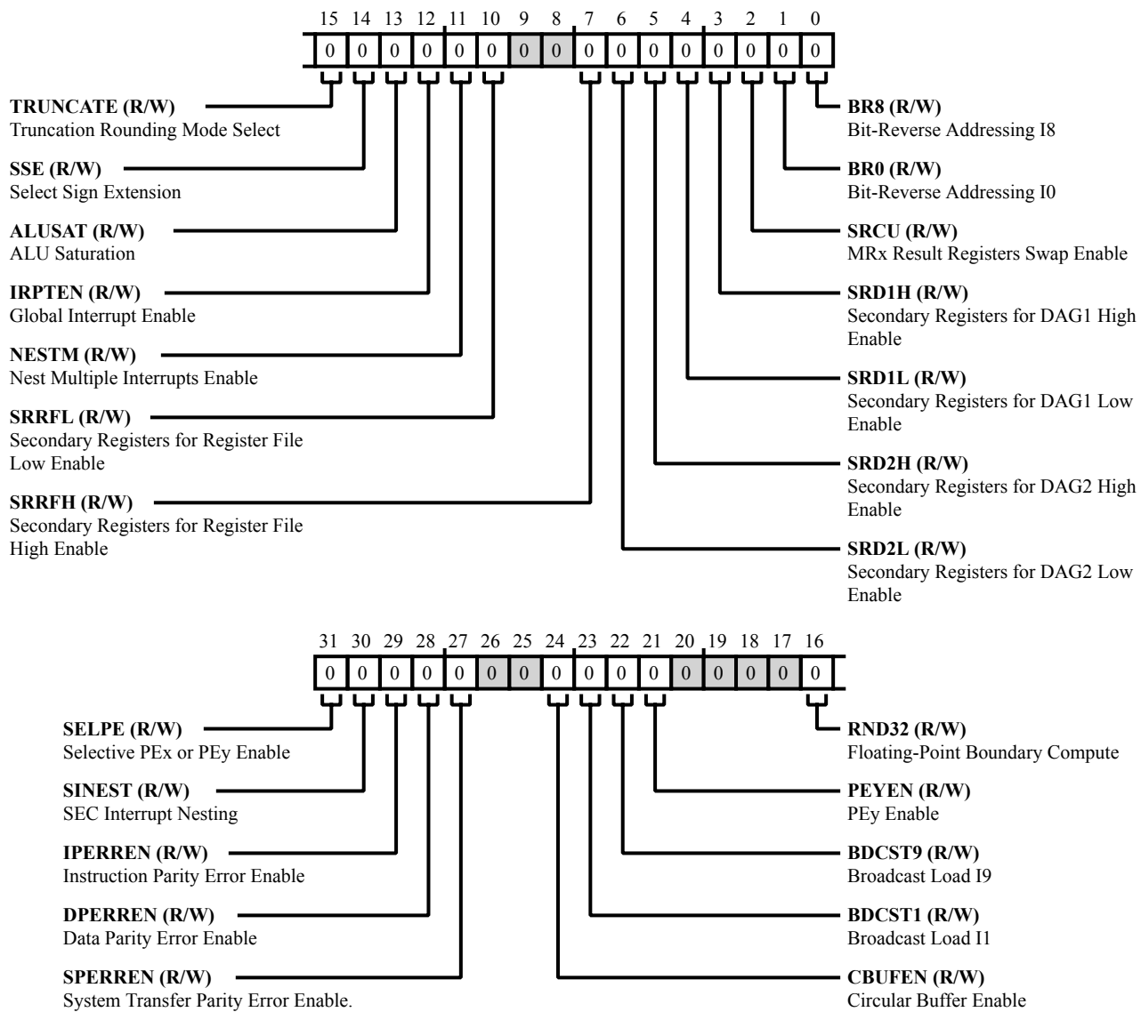
Figure 28-18: REGF_MODE1 Register Diagram
