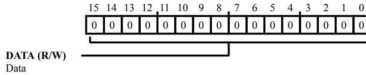
Figure 28-32: REGF_MS2F Register Diagram
