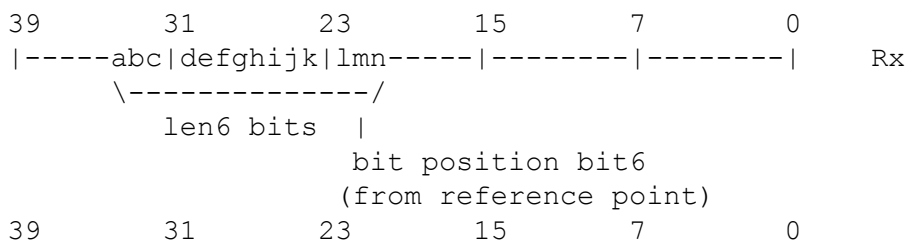
Figure 23-3: Field Alignment
