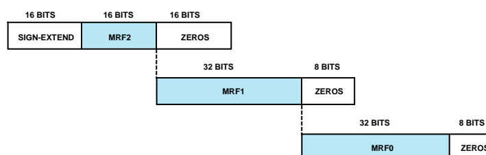
Figure 3-3: MR to Data Register Transfers Formats
