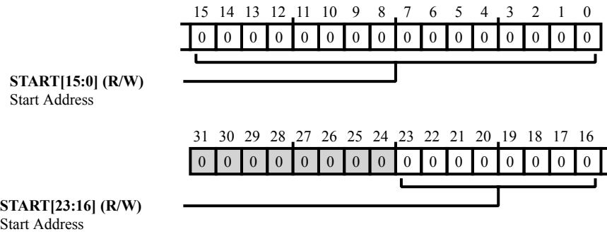
Figure 31-27: SHDBG_PSA2S Register Diagram
