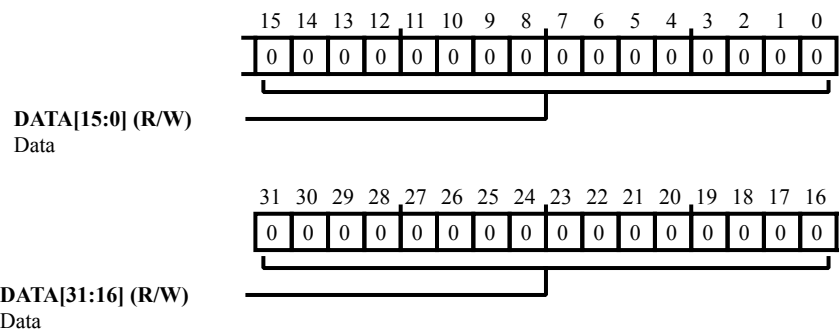
Figure 28-6: REGF_EMUCLK Register Diagram
