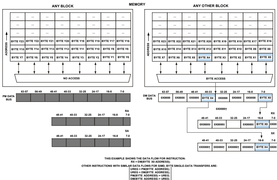
Figure 7-9: Byte Addressing of Single-Data in SIMD Mode
