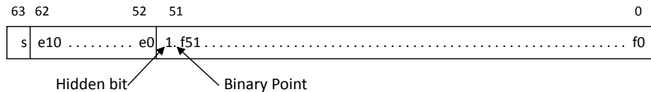
Figure 27-2: IEEE 64-bit Double Precision floating point format
