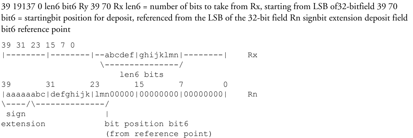
Figure 23-2: Field Alignment
