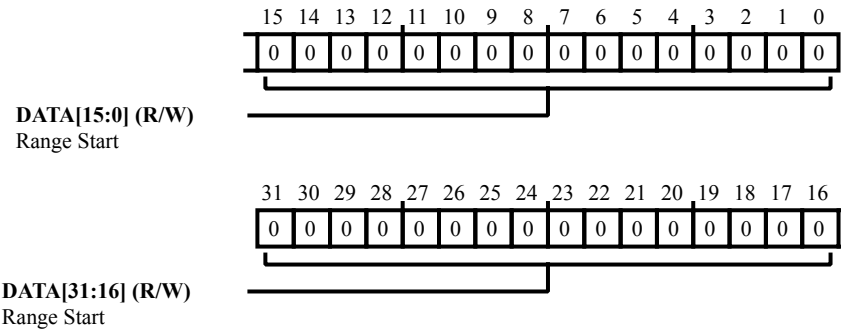
Figure 32-20: SHL1C_RANGE_START7 Register Diagram
