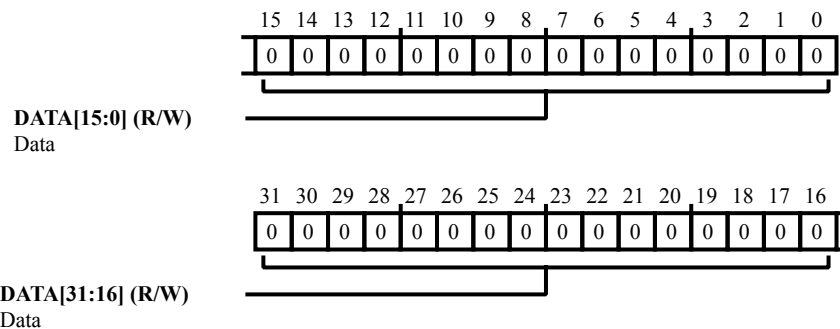
Figure 28-15: REGF_LCNTR Register Diagram
