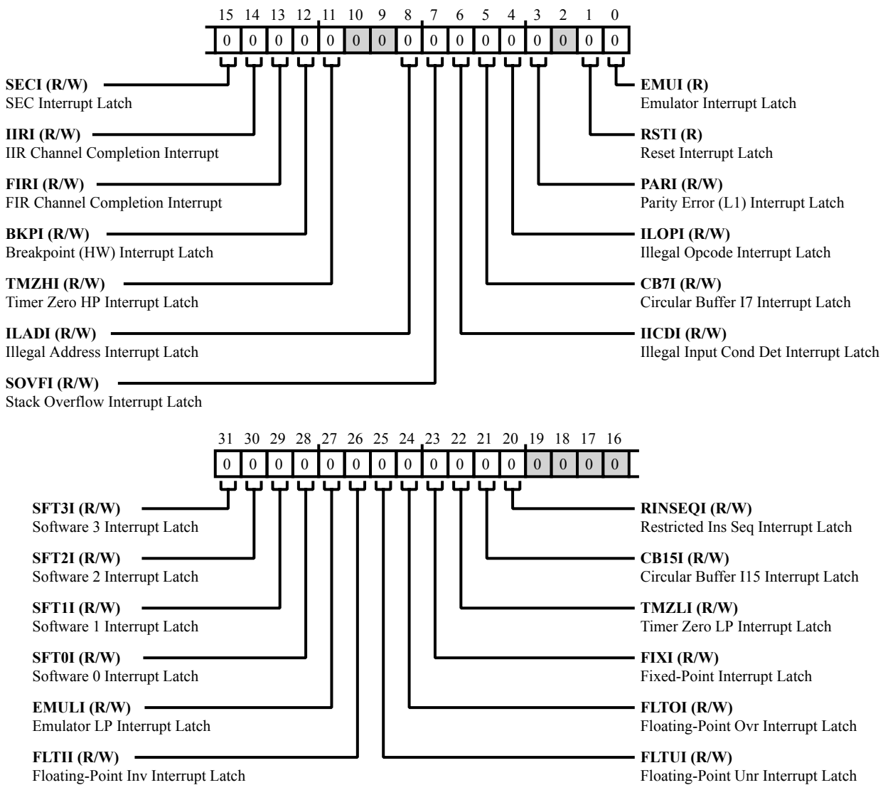
Figure 28-12: REGF_IRPTL Register Diagram
