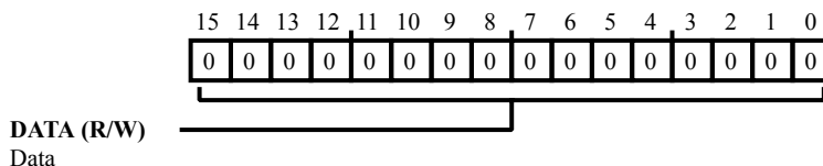
Figure 28-26: REGF_MR2F Register Diagram
