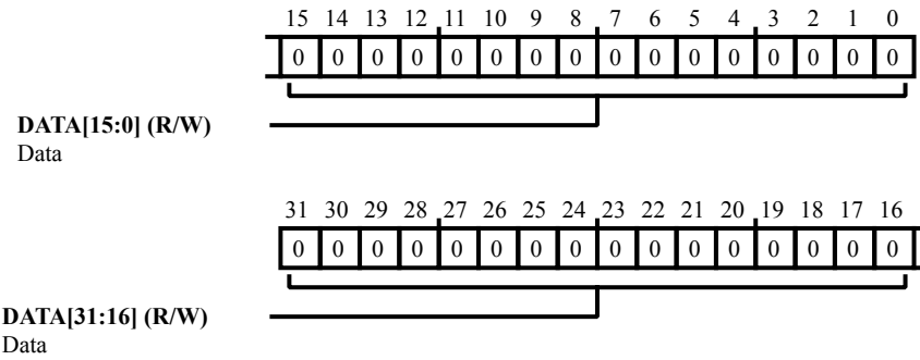
Figure 31-19: SHDBG_M3ADDR Register Diagram
