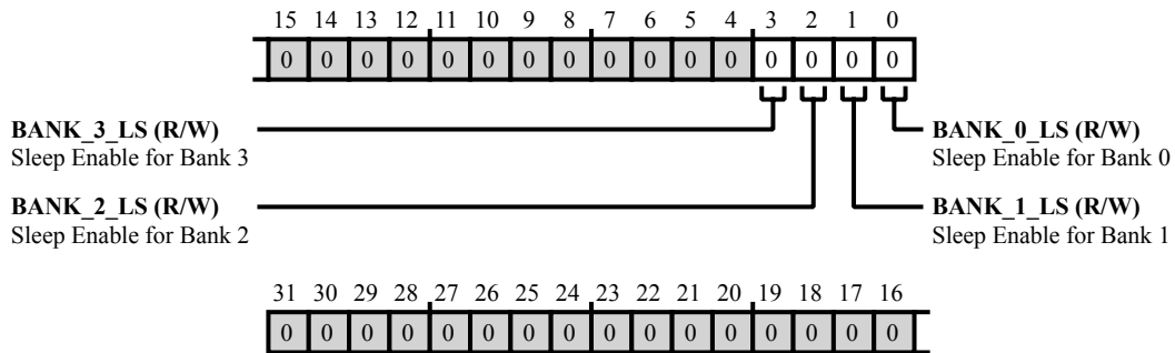
Figure 29-5: CMMR_PWR_L1_LS_CTL Register Diagram
