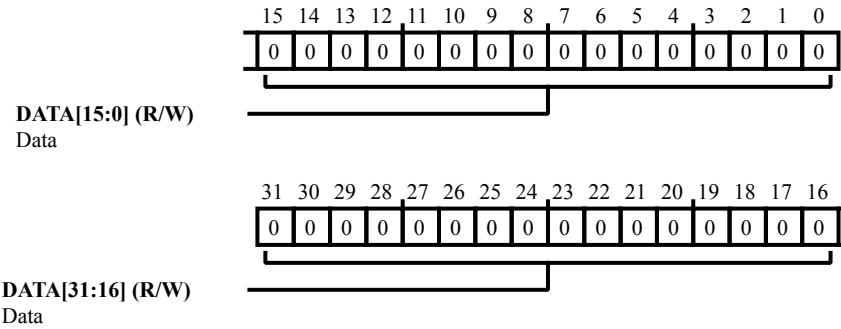
Figure 31-33: SHDBG_SECI_ID Register Diagram
