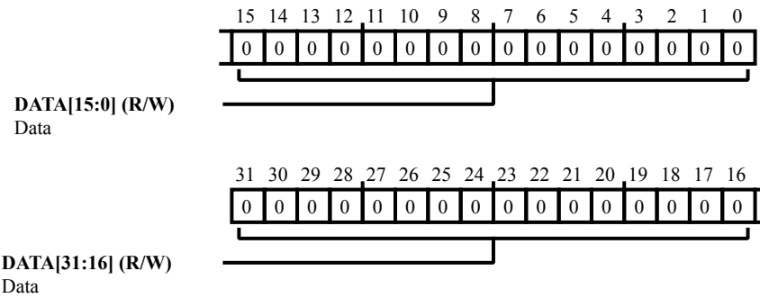
Figure 28-13: REGF_I[n] Register Diagram
