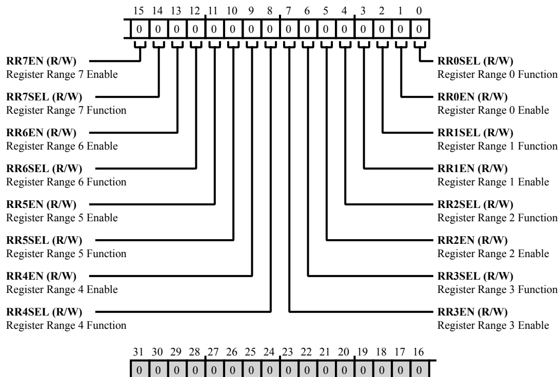
Figure 32-2: SHL1C_CFG2 Register Diagram
