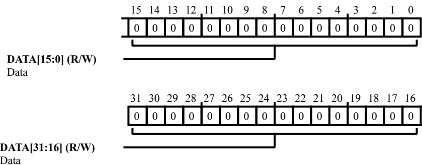
Figure 28-43: REGF_USTAT1 Register Diagram
