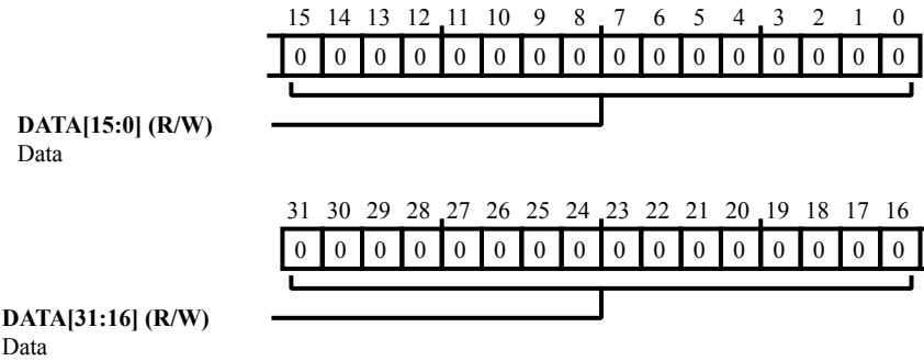
Figure 28-14: REGF_LADDR Register Diagram
