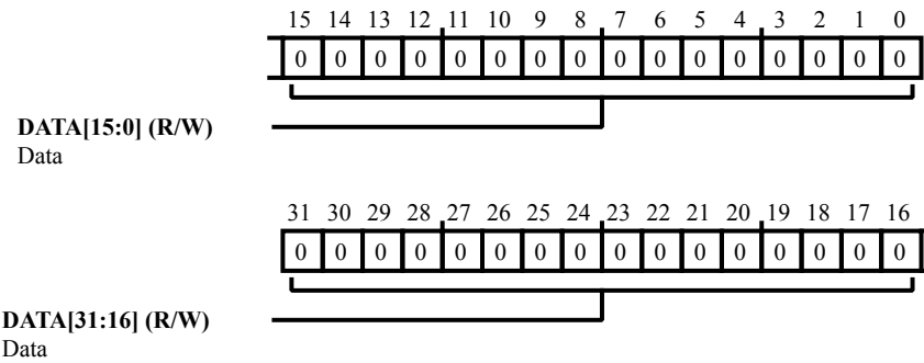
Figure 28-44: REGF_USTAT2 Register Diagram
