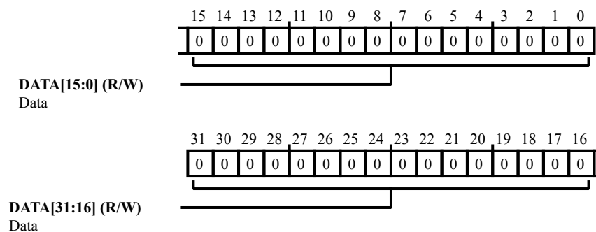
Figure 28-7: REGF_EMUCLK2 Register Diagram
