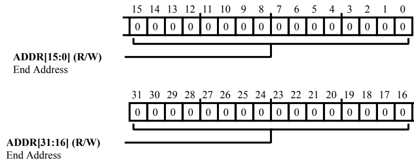
Figure 29-2: CMMR_PFB_NOCHRT0_END Register Diagram
