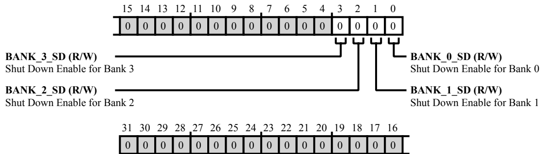
Figure 29-6: CMMR_PWR_L1_SD_CTL Register Diagram
