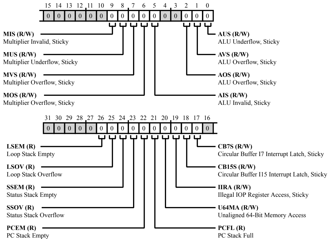
Figure 28-39: REGF_STKYX Register Diagram
