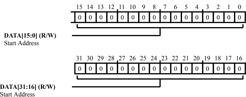
Figure 30-3: SHBTB_LOCK_START Register Diagram
