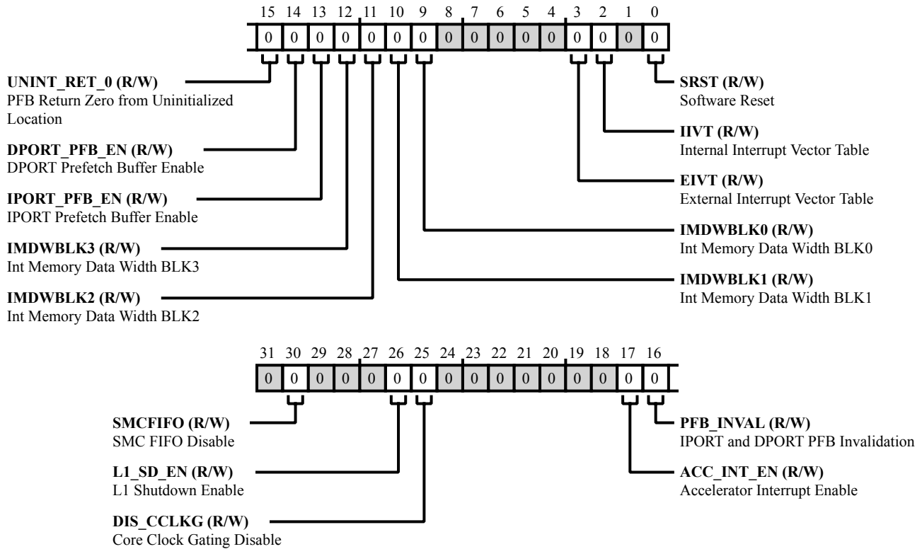
Figure 29-7: CMMR_SYSCTL Register Diagram
