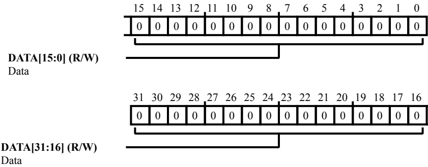
Figure 28-29: REGF_MS1B Register Diagram
