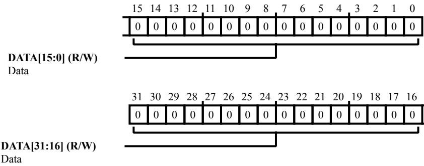
Figure 28-42: REGF_TPERIOD Register Diagram
