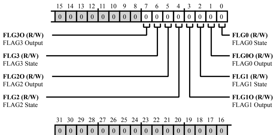
Figure 28-9: REGF_FLAGS Register Diagram
