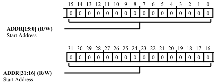
Figure 29-3: CMMR_PFB_NOCHRT0_ST Register Diagram
