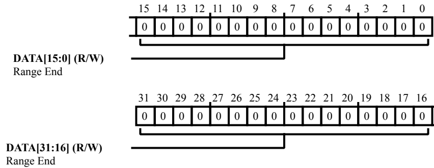
Figure 32-9: SHL1C_RANGE_END4 Register Diagram
