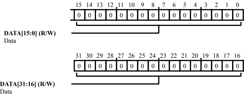
Figure 28-3: REGF_B[n] Register Diagram
