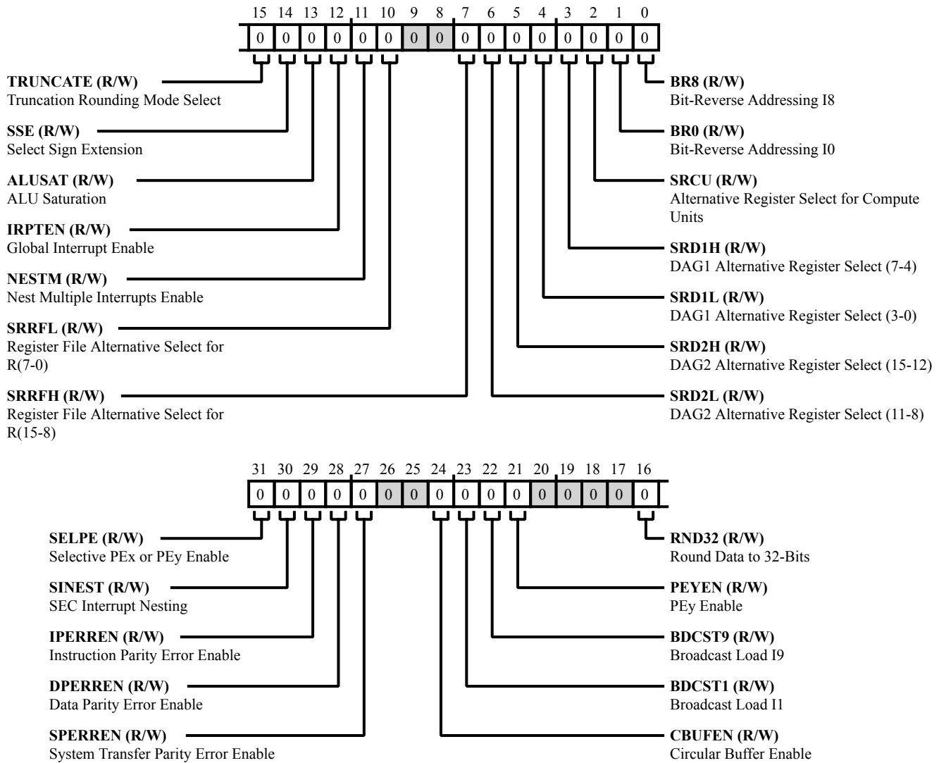
Figure 28-19: REGF_MODE1STK Register Diagram
