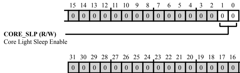
Figure 29-4: CMMR_PWR_GLB_CTL Register Diagram
