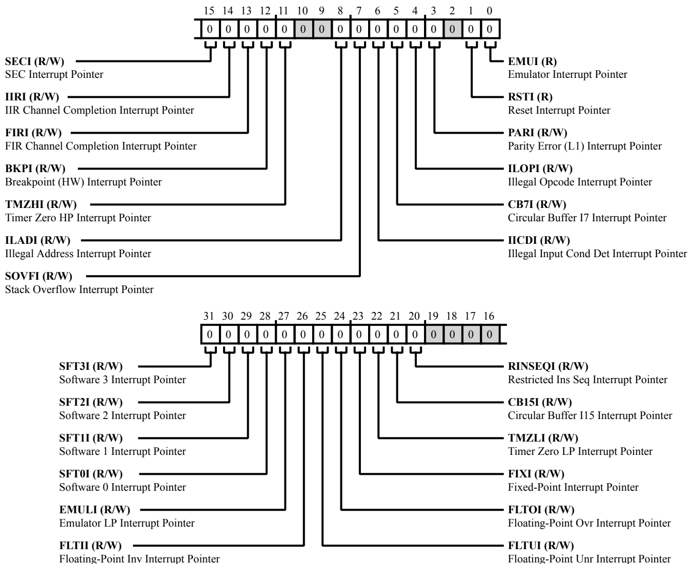
Figure 28-11: REGF_IMASKP Register Diagram
