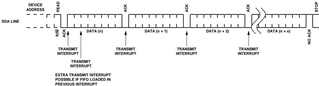
Figure 23. I 2 C Slave Tx Interrupt Details
