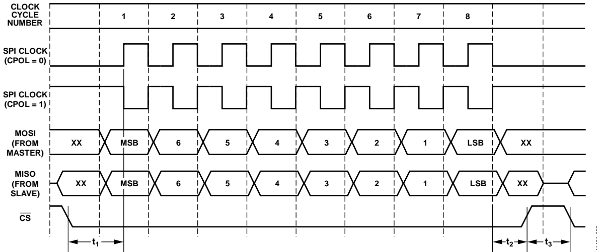
Figure 24. SPI Transfer Protocol, CPHA = 0
