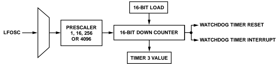
Figure 28. Watchdog Timer Block Diagram
