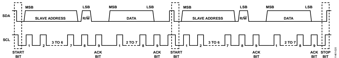
Figure 22. I 2 C Repeated Start Sequence
