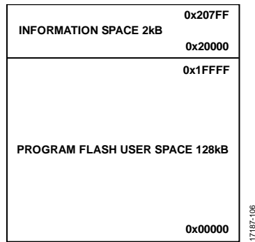
Figure 6. ADuCM331WFS (128 kB) Program Flash Memory Map
