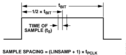
Figure 34. LIN Bit Sample Spacing
