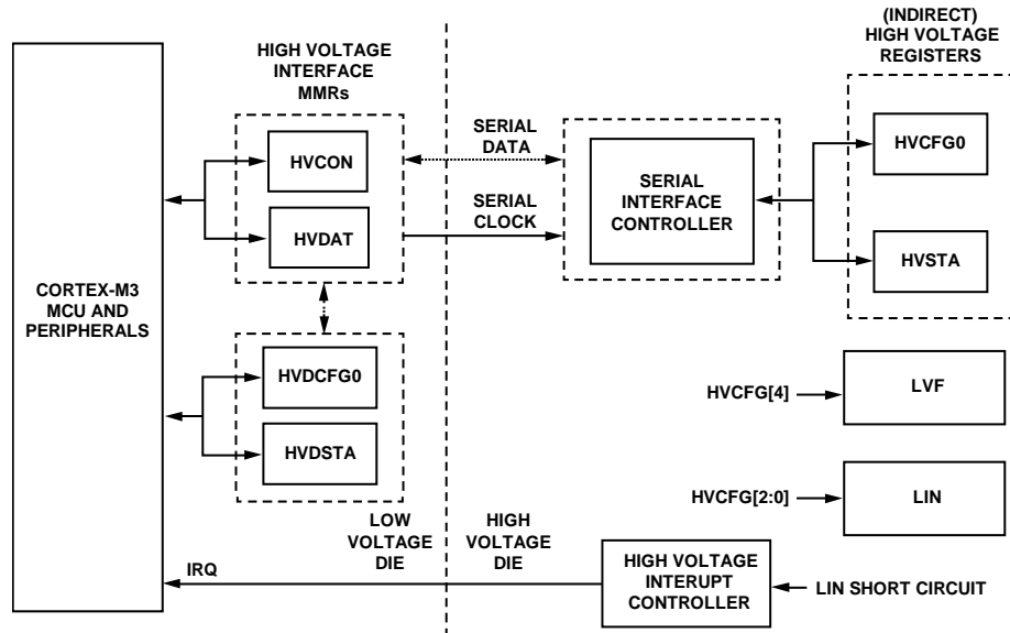
Figure 29. High Voltage Interface, Top Level Block Diagram
