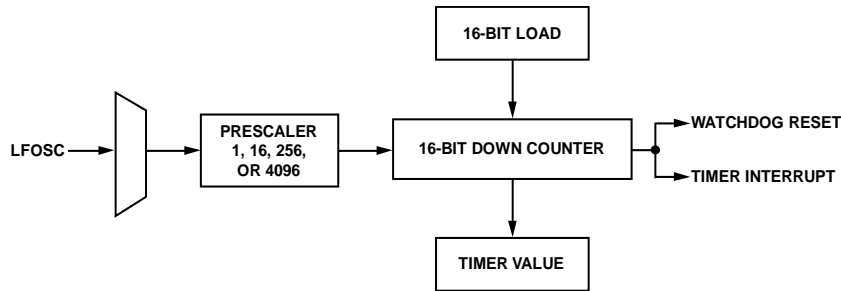
Figure 23. Watchdog Timer Block Diagram
