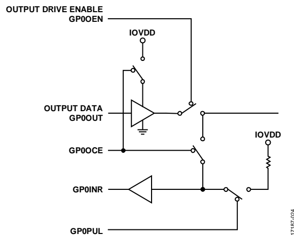
Figure 24. GPIO Block Diagram
