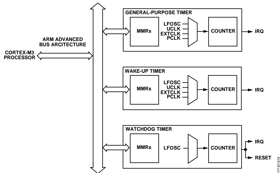
Figure 19. Timer Synchronization Block Diagram
