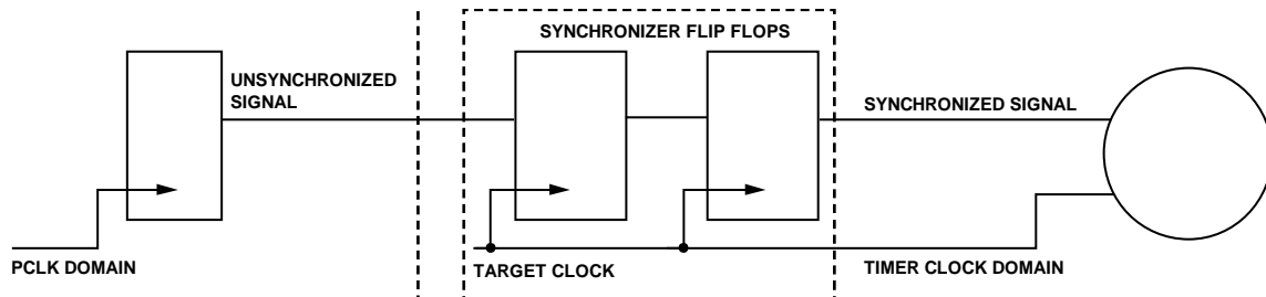
Figure 20. Synchronizer for Signals Crossing Clock Domains
