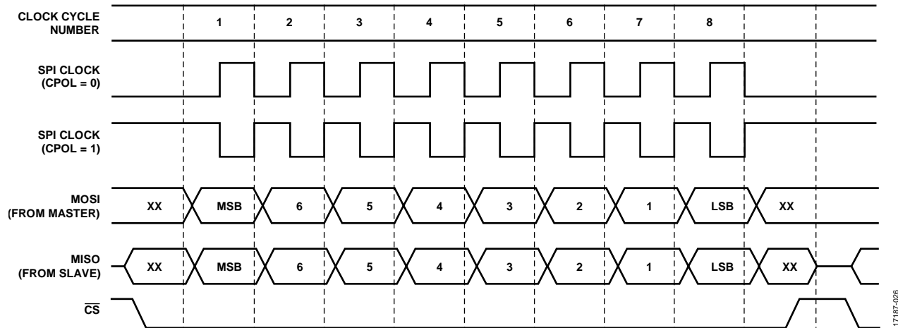
Figure 26. SPI Transfer Protocol, CPHA = 0
