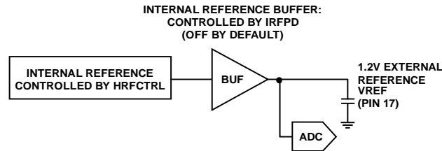
Figure 16. ADC Reference Configuration
