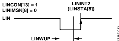
Figure 33. Wake-Up Interrupt
