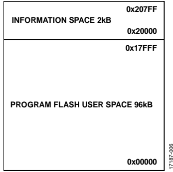
Figure 5. ADuCM330WFS (96 kB) Program Flash Memory Map
