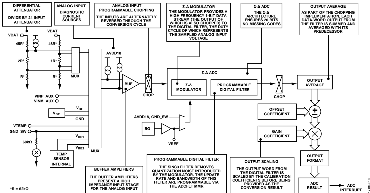
Figure 10. Voltage and Temperature ADC (ADC1) Top Level Overview
