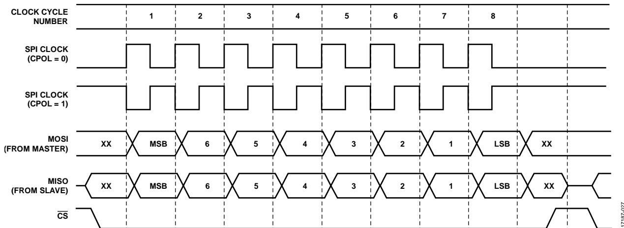
Figure 27. SPI Transfer Protocol, CPHA = 1
