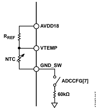
Figure 17. Internal Ground Switch Configuration
