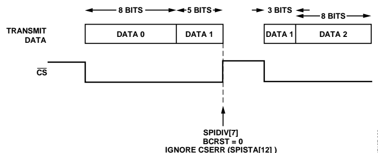
Figure 28. Serial Peripheral Interface, Erroneous Deassertion of Chip Select Diagram
