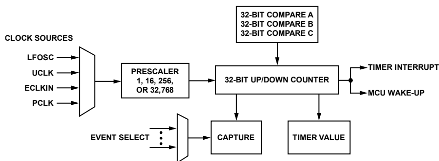
Figure 22. Wake-Up Timer Block Diagram
