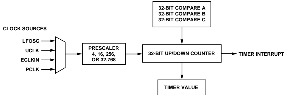
Figure 21. General-Purpose Timers Block Diagram
