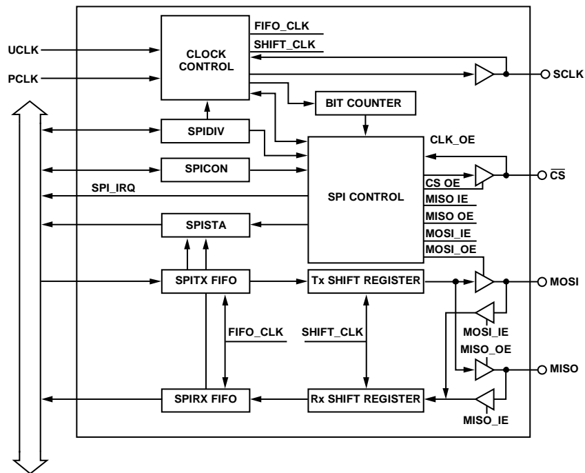
Figure 25. SPI Block Diagram
