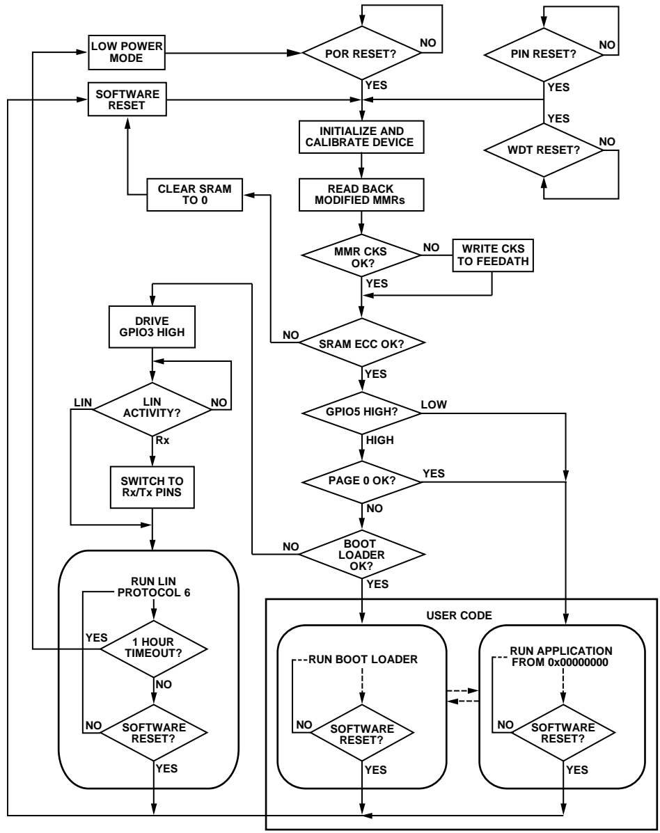
Figure 3. Kernel Flowchart
