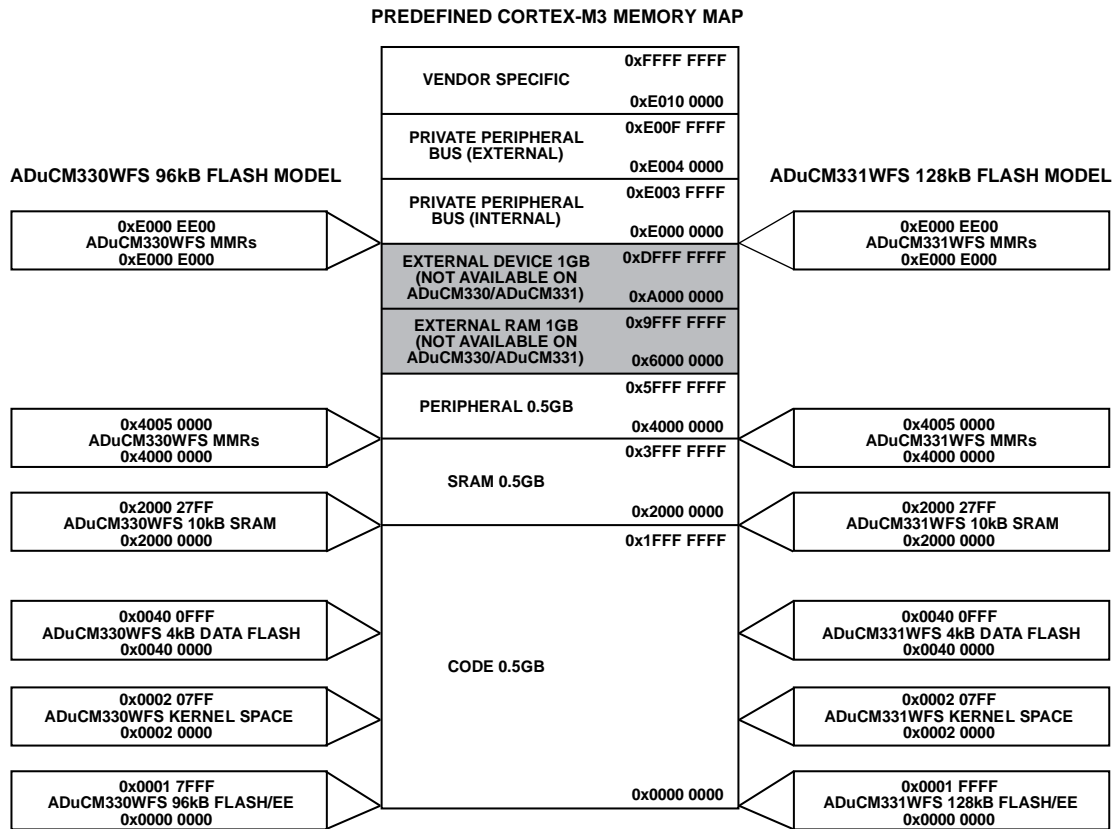
Figure 4. ADuCM330WFS/ADuCM331WFS Memory Map Diagram
