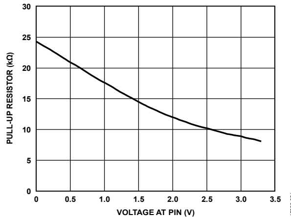
Figure 22. GPIO Pull-Up Resistor Value
