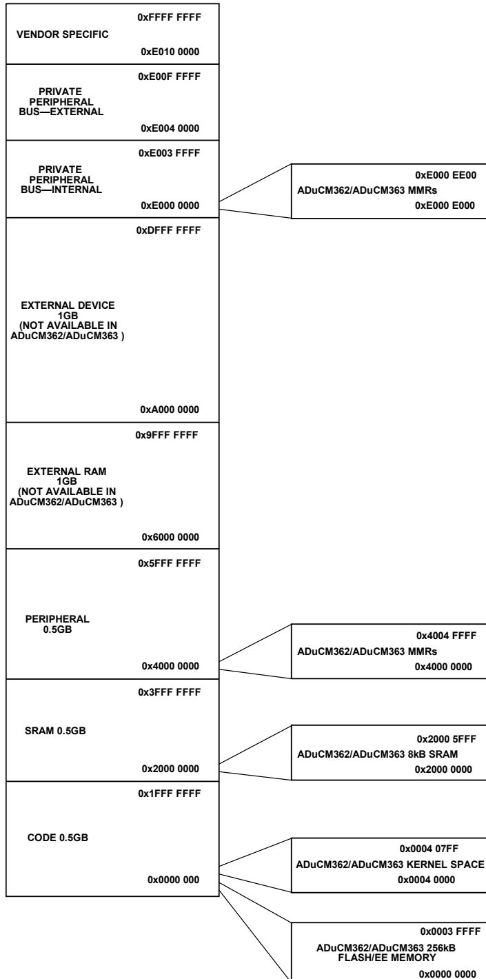
Figure 3. ADuCM362/ADuCM363 Cortex-M3 Memory Map Diagram Rev. A | Page 8 of 175
