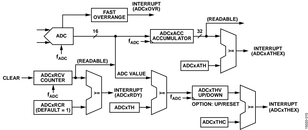
Figure 16. ADC Accumulator/Comparator/Counter Functional Diagram
