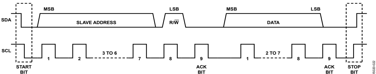
Figure 23. Typical I 2 C Transfer Sequence
