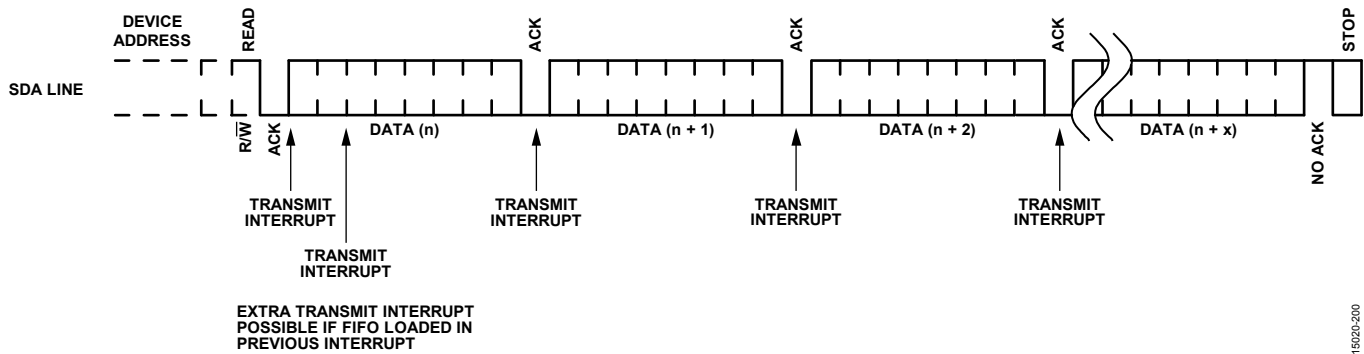
Figure 26. I 2 C Slave Tx Interrupt Details
