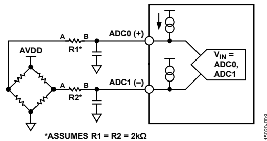
Figure 10. Example Circuit Using Diagnostic Current Sources
