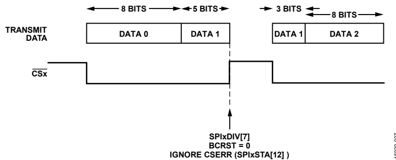
Figure 29. SPI Communication: Midbyte Stall
