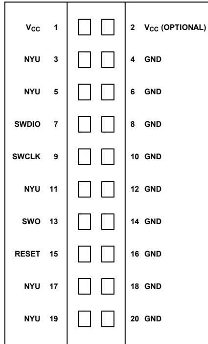
Figure 41. SWD 20-Pin Connector Pinout
