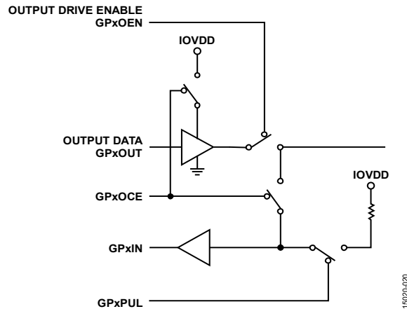
Figure 21. GPIO Structure
