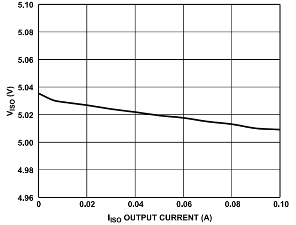
Figure 10. V_{ISO} vs. I_{ISO} Output Current, Input = 5 V, V_{ISO} = 5 V
