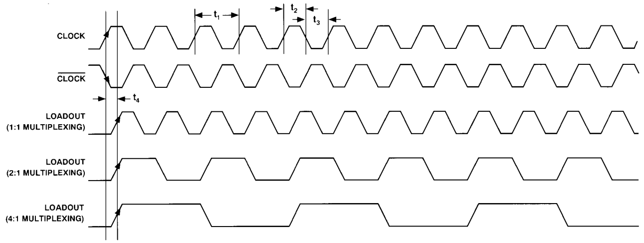
Figure 2. LOADOUT vs. Pixel Clock Input (CLOCK, \overline{\text{CLOCK}} )
