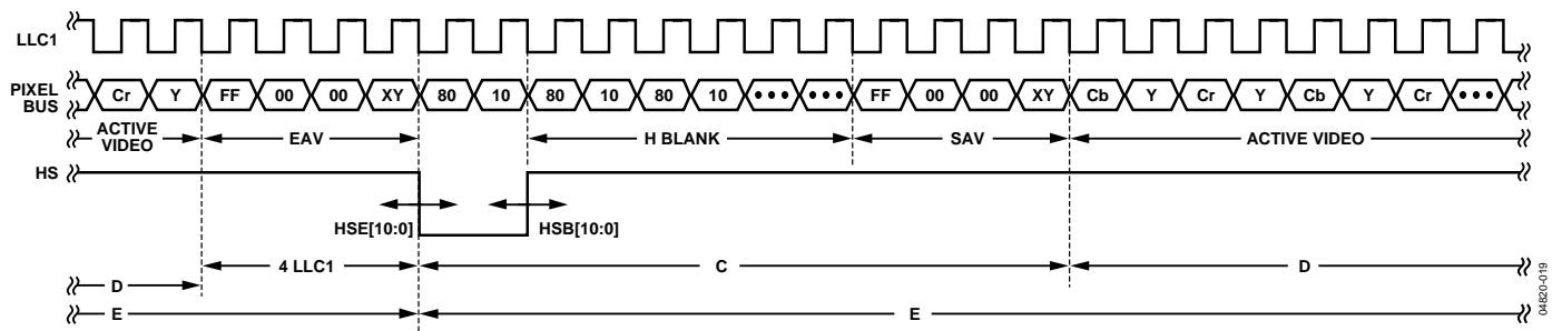
Figure 19. HS Timing
