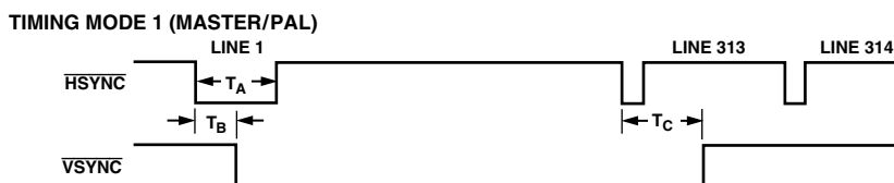
Figure 51. Timing Register 1
