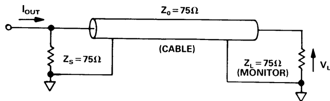
Figure 3. Doubly Terminated 75Ω Load
