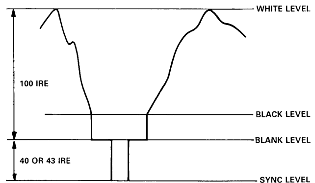
Figure 1. RGB Video Waveform
