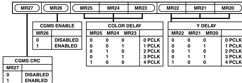
Figure 22. Mode Register 2
