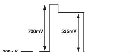
Figure 95. PS RGB Output Levels
