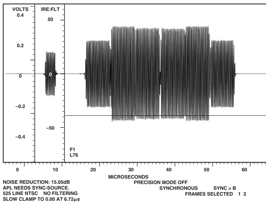
Figure 106. NTSC Chroma
