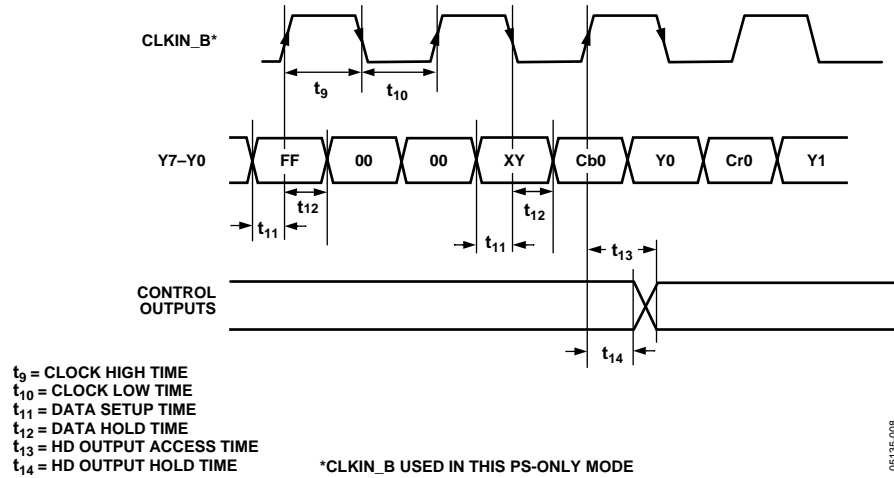
Figure 8. PS Only, 4:2:2 8-Bit Interleaved at 27 MHz EAV/SAV Input Mode (Input Mode 100)
