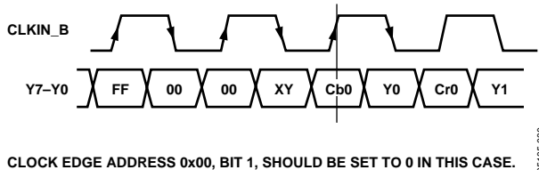
Figure 53. Input Sequence in PS Bit-Interleaved Mode (EAV/SAV)
