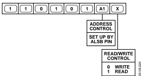
Figure 44. ADV7322 Slave Address = 0xD4
