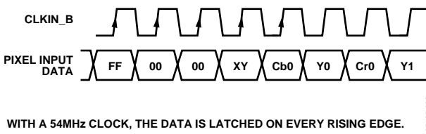
Figure 55. Input Sequence in PS Bit-Interleaved Mode (EAV/SAV)
