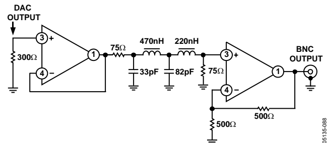
Figure 86. Example of Output Filter for HDTV, 2x Oversampling
