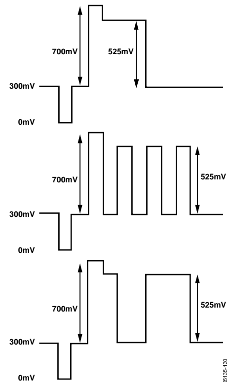
Figure 129. SD RGB Output Levels—RGB Sync Enabled
