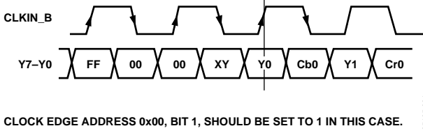
Figure 54. Input Sequence in PS Bit-Interleaved Mode (EAV/SAV)
