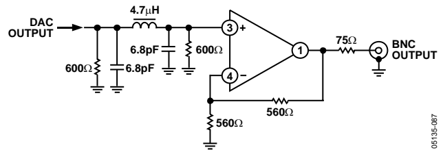
Figure 85. Example of Output Filter for PS, 8x Oversampling
