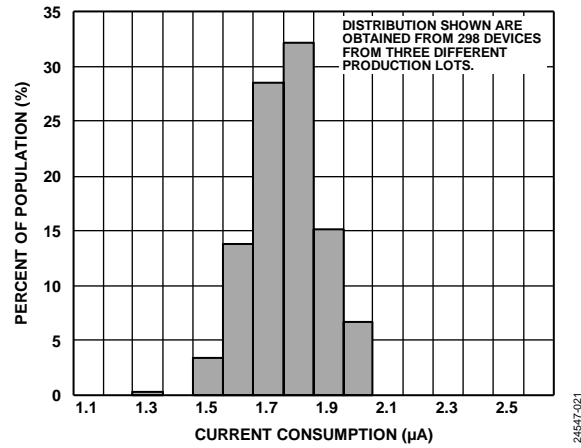
Figure 21. Current Consumption at 25°C, Instant On Mode, V_S = 3.3 V
