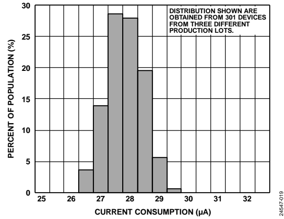
Figure 19. Current Consumption at 25°C, Normal Mode, 2560 Hz Output Data Rate, V_S = 3.3 V
