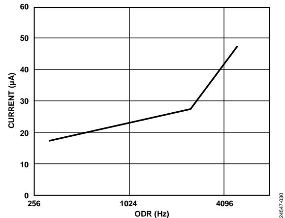
Figure 30. Typical Measurement Mode Current vs. ODR
