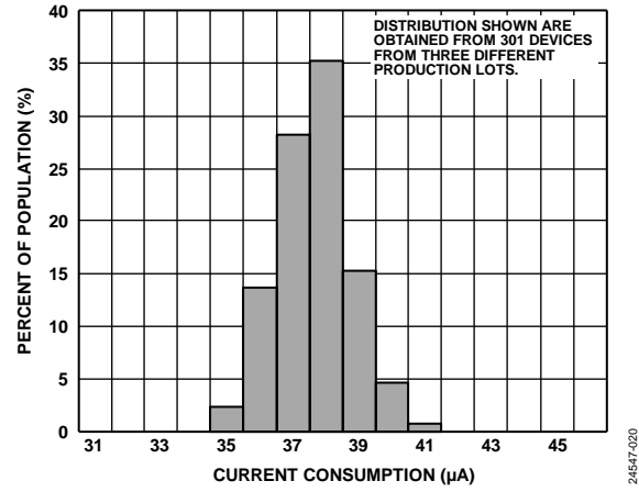
Figure 20. Current Consumption at 25°C, Low Noise Mode, 2560 Hz Output Data Rate, V_S = 3.3 V
