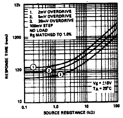
RESPONSE TIME vs SOURCE RESISTANCE
