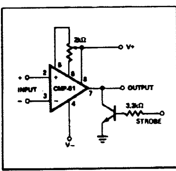
OFFSET TRIMMING AND STROBE CIRCUIT
