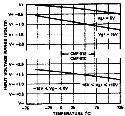
INPUT VOLTAGE RANGE vs TEMPERATURE
