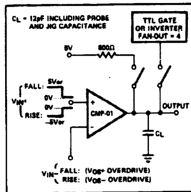
RESPONSE TIME TEST CIRCUIT
