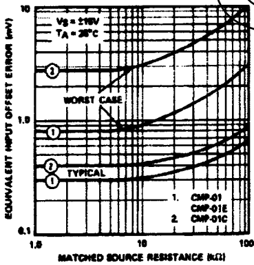
INPUT OFFSET ERROR vs SOURCE RESISTANCE
