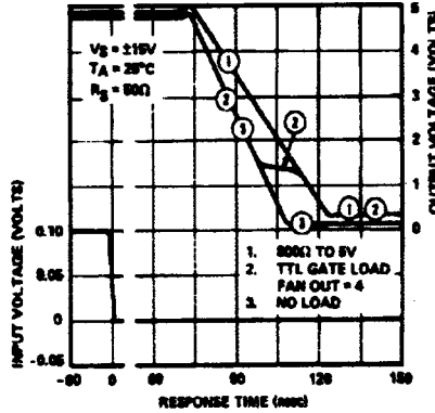
RESPONSE TIME, 100mV STEP, 5mV OVERDRIVE, VARIOUS LOADS
