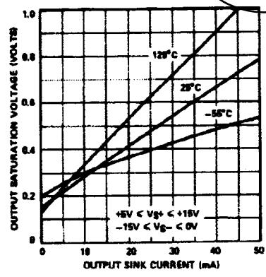
SATURATION VOLTAGE vs SINK CURRENT
