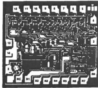
DIE SIZE 0.080 x 0.067 inch, 5,360 sq. mils (2.032 x 1.702 mm, 3.458 sq. mm)
