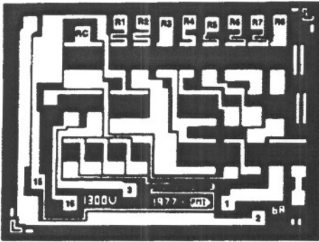
DIE SIZE .090 x .064 inch, 5760 sq. mils (2.286 x 1.701 mm, 3.888 sq. mm)
