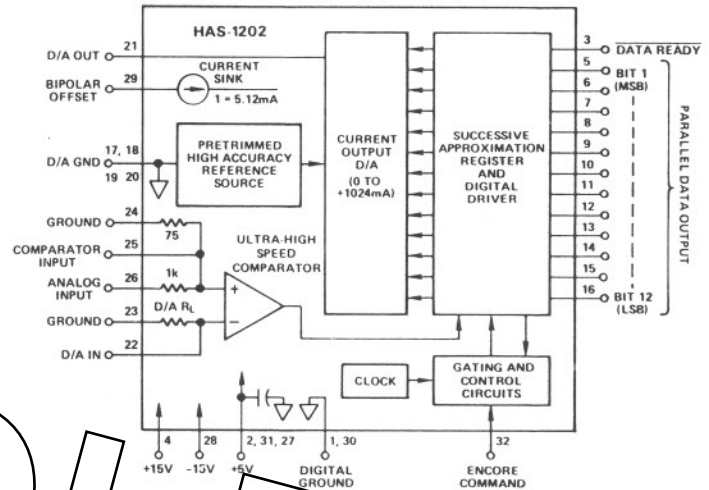
HAS-0802/1002/1202 FUNCTIONAL BLOCK DIAGRAM
