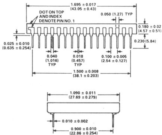
HY32A 32-Pin Hybrid Package
