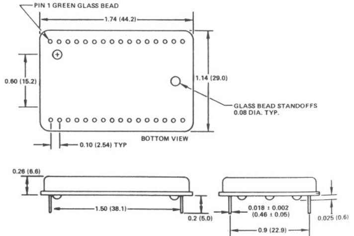
HY32B 32-Pin Hybrid Package
