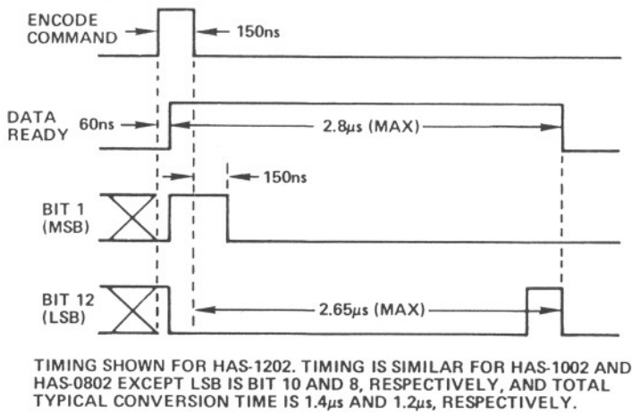
Figure 1. Timing Diagram (Typical)
