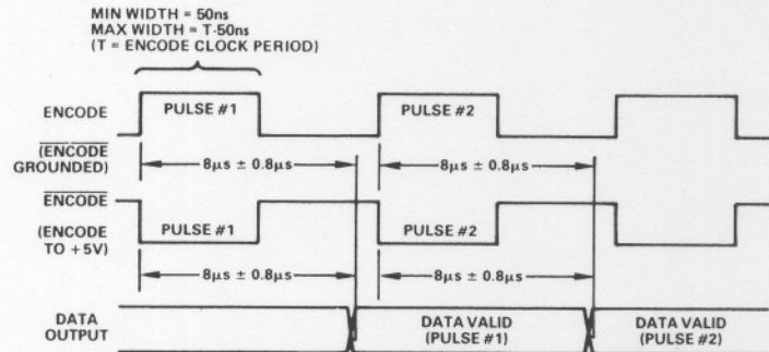
Figure 1. HAS-1409KM and HAS-1409LM A/D Timing Diagram
