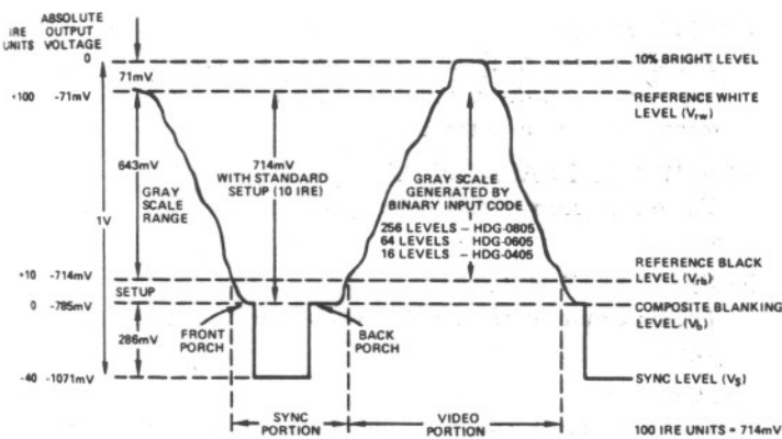
Figure 1. Composite Output Waveform
