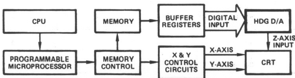
Typical Raster Scan Display System
