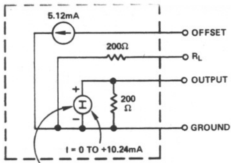
CURRENT CONTROLLED BY DIGITAL INPUT CODE
