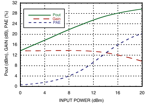
Power Compression @ 12 GHz
