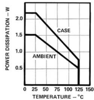
Figure 2. Power Derating
