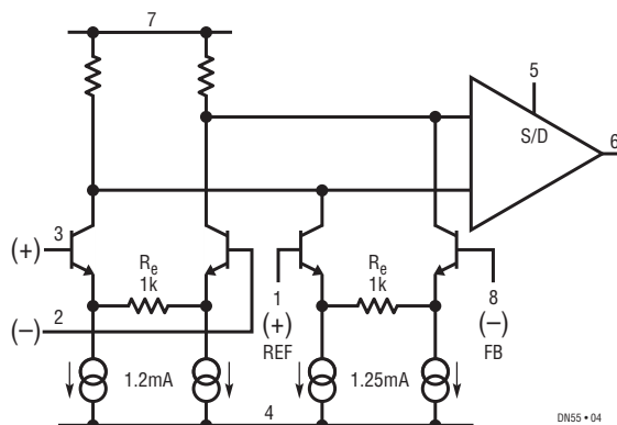
Figure 4. LT1193 Simplified Schematic
