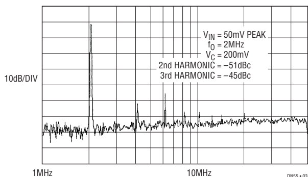
Figure 3. VCA Output Spectrum
