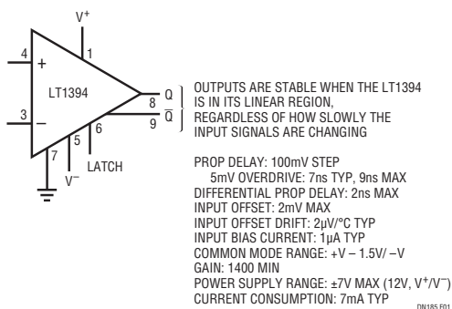
Figure 1. The LT1394 at a Glance
