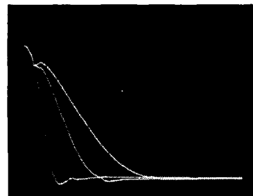
1525A/1527A C_L = 1kF, = 5kF, = 10kF V = 2.5V/DIV H = 100ns/DIV
