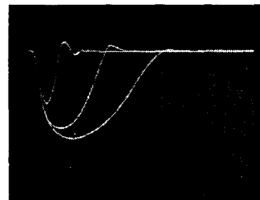
OUTPUT CURRENT 100mA/DIV 100ns/DIV
