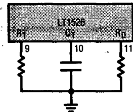
Oscillator Connections
