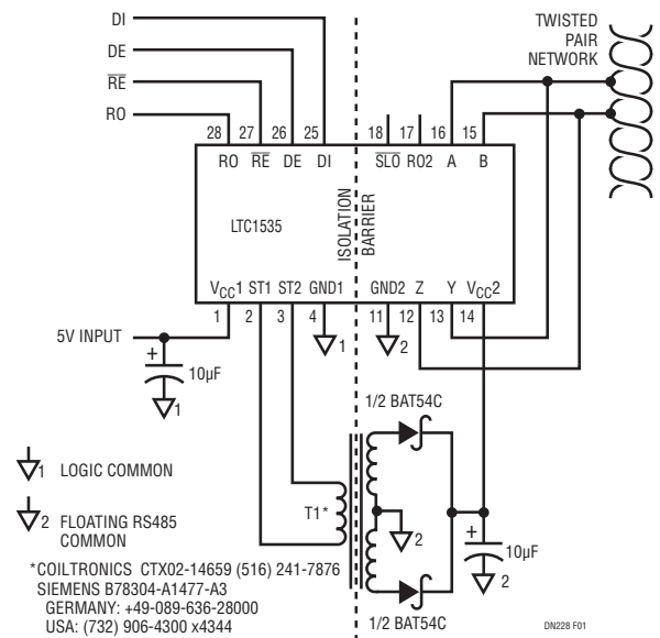
Figure 1. Fully Isolated RS485 Port
