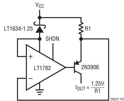
Figure 4. Current Source
