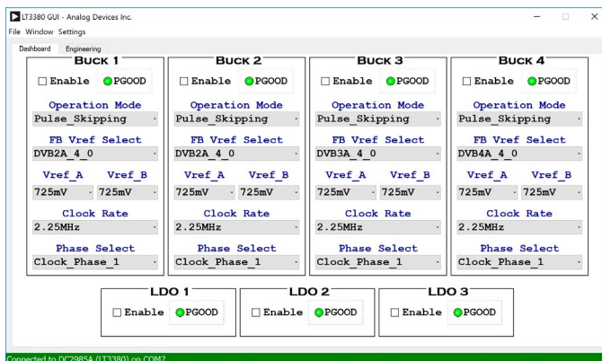
Figure 6. LT3380 GUI Dashboard Tab
