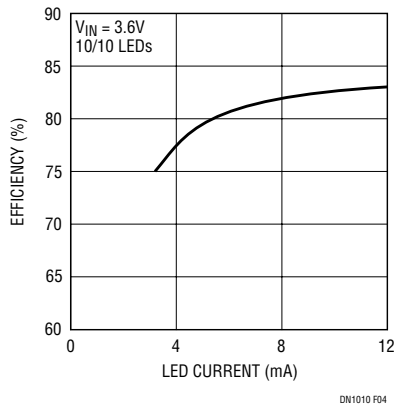
Figure 4. Efficiency vs LED Current, Circuit of Figure 3
