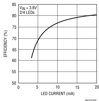
Figure 2. Efficiency vs LED Current, Circuit of Figure 1
