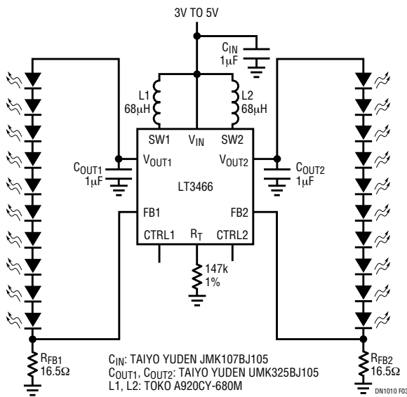
Figure 3. Li-Ion to 10/10 White LEDs
