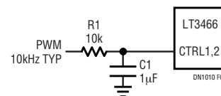
Figure 6. Filtered PWM Dimming
