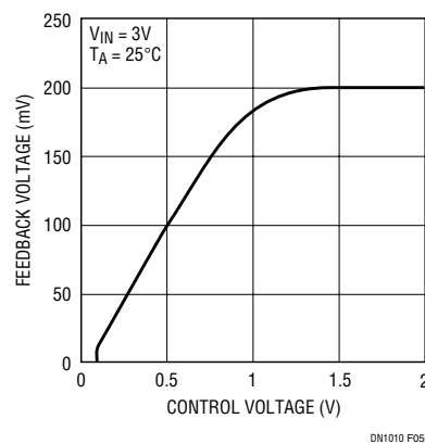
Figure 5. Feedback Voltage vs V_{CTRL}
