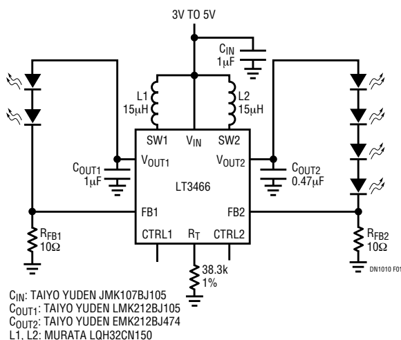
Figure 1. Li-Ion to 2/4 White LEDs
