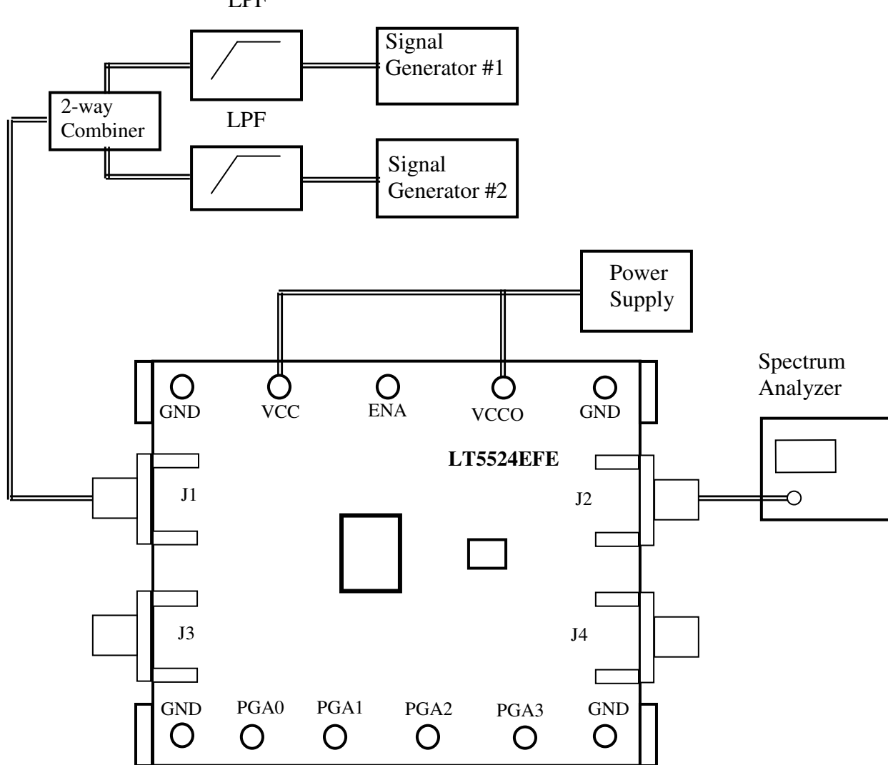
Figure 3. Test & Measurement Setup for Single Ended Input & Single Ended Output Demo Circuit.
