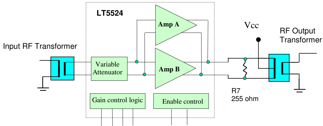
Figure 2. Block Diagram of the DC807A Demo Circuit with Type A Input and with Type B Output Configuration.
