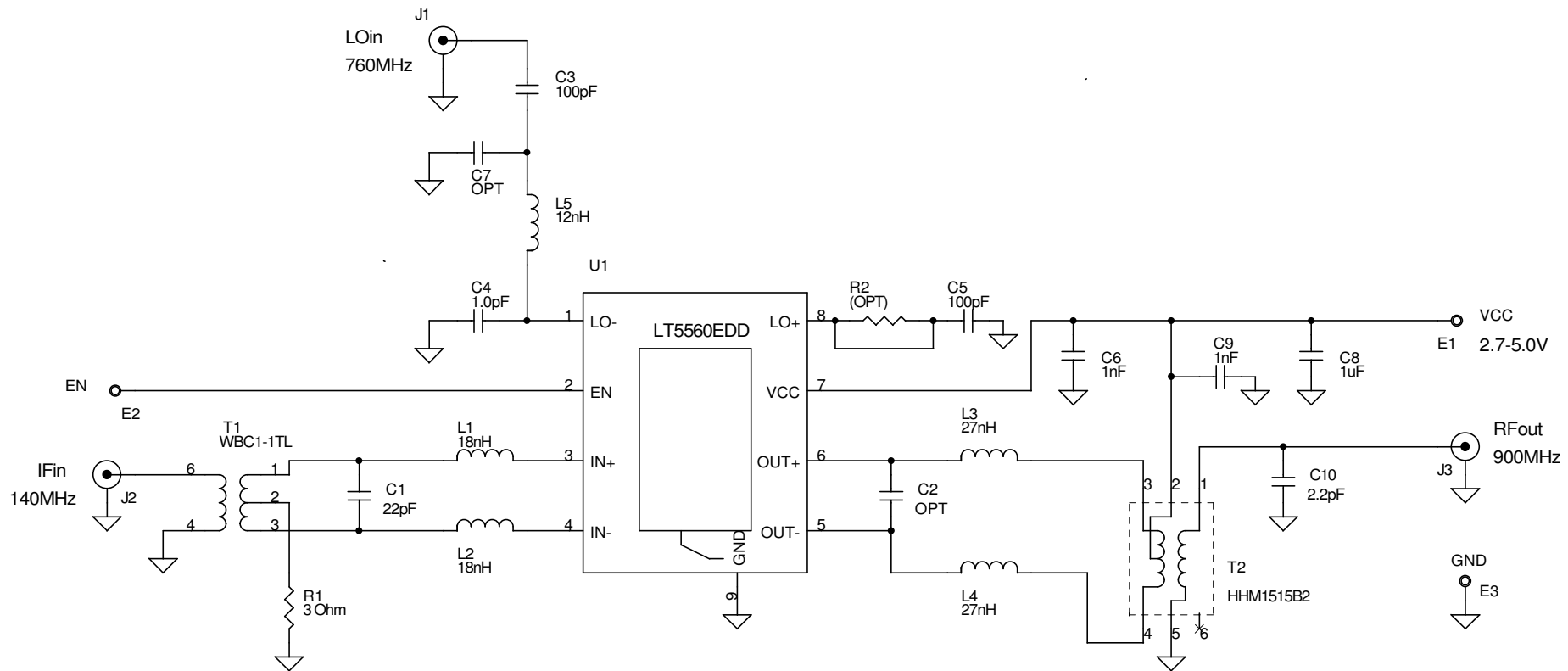
T1 Circuit Diagram
