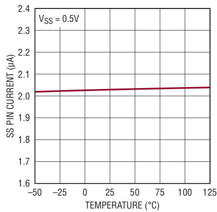
Soft-Start Current
