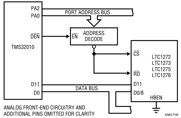
Figure 46. LTC1272/LTC1273/LTC1275/LTC1276 to TMS32010 DSP Processor Parallel Interface
