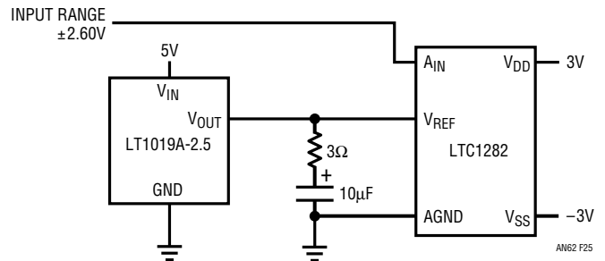
Figure 25. Ultra-Low Full-Scale Drift LTC1282 3V Analog-to-Digital Converter
